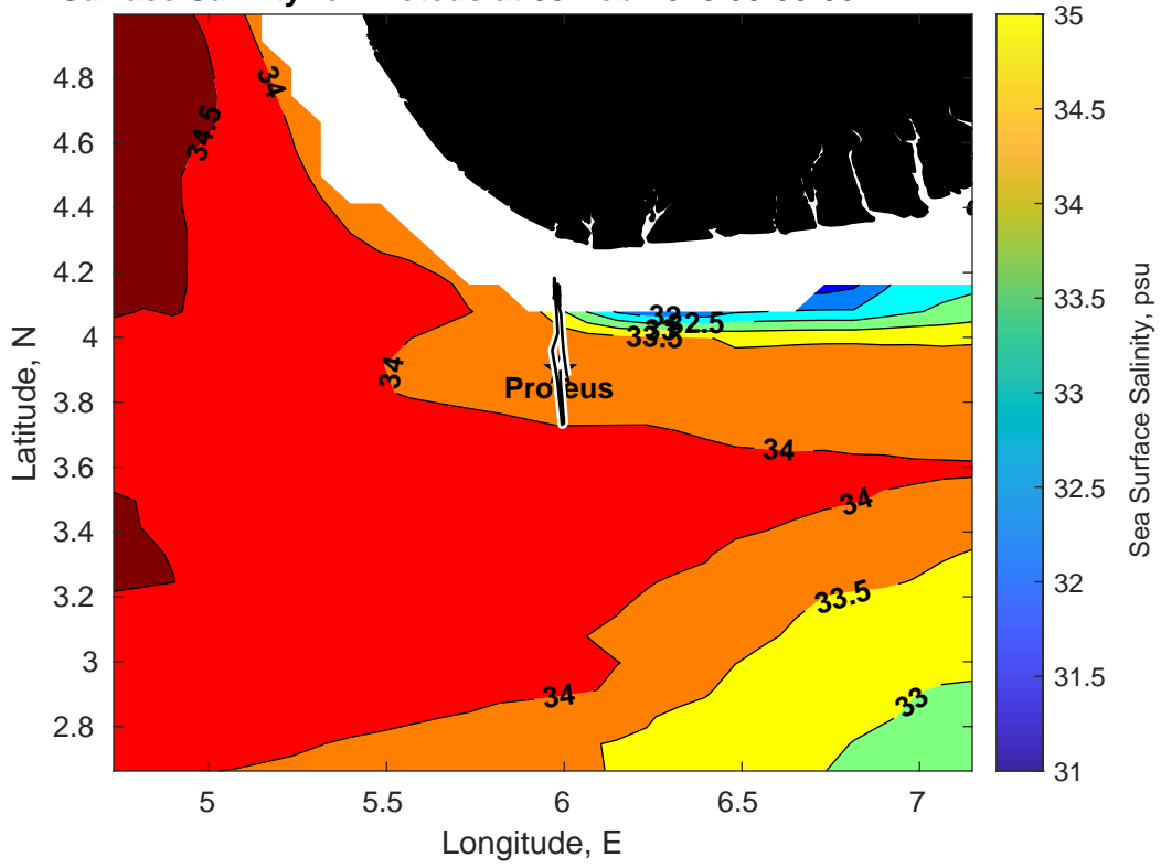
Surface Salinity for Proteus at 03-Feb-2025 00:00:00
