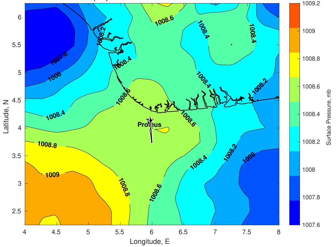
Surface Pressure (mb) for Proteus at 04-Feb-2025 00:00:00
