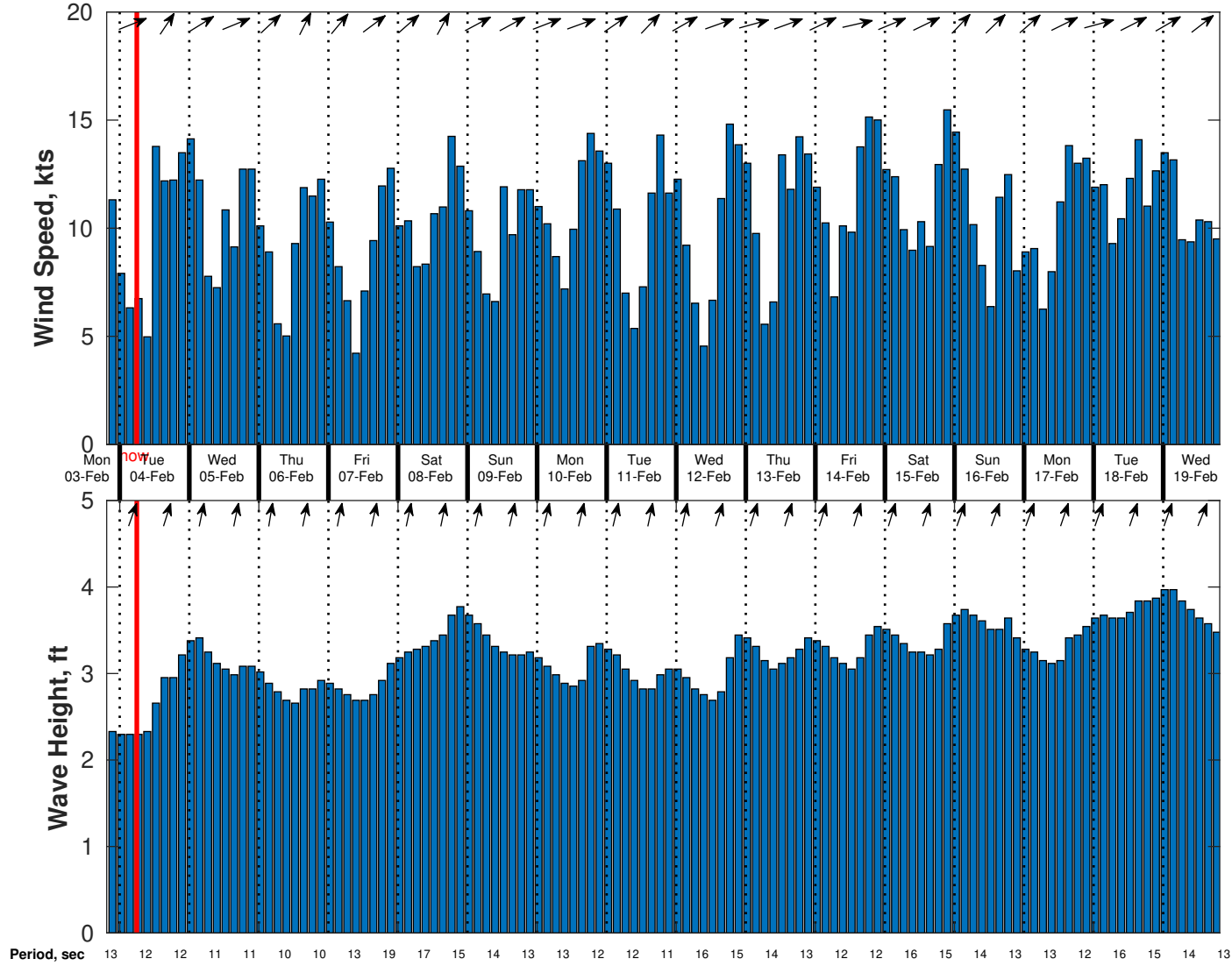
Wind & Wave Forecast for Proteus from 03-Feb-2025 20:00:00 to 19-Feb-2025 20:00:00
