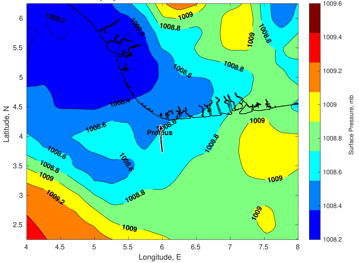
Surface Pressure (mb) for Proteus at 06-Feb-2025 00:00:00
