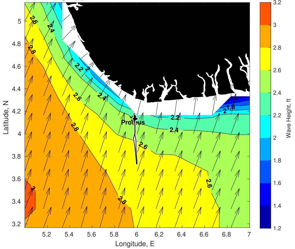
Wave Height (ft) for Proteus at 04-Feb-2025 09:00:00
