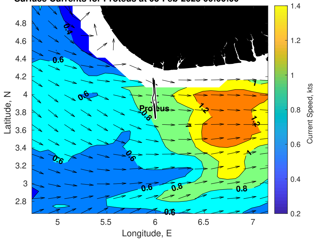
Surface Currents for Proteus at 03-Feb-2025 00:00:00
