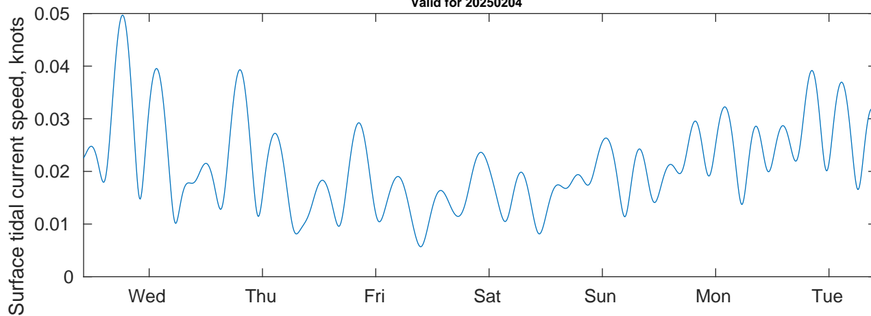
Tidal Currents and Heights for TOTAL Namibia GTS at 20250204
