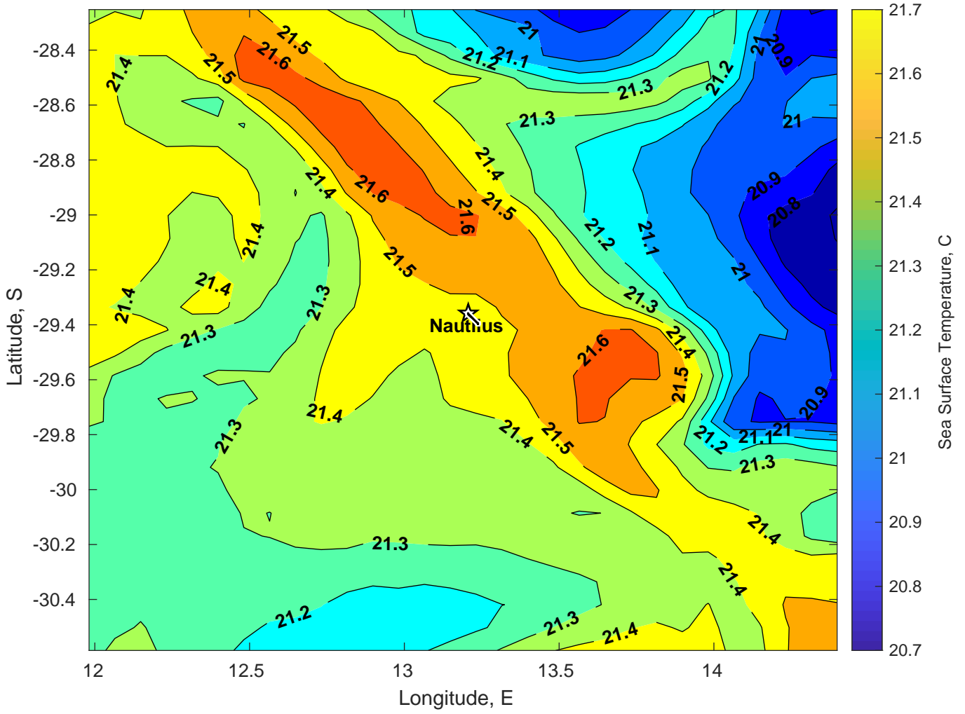
SST for Nautilus at 04-Feb-2025 00:00:00
