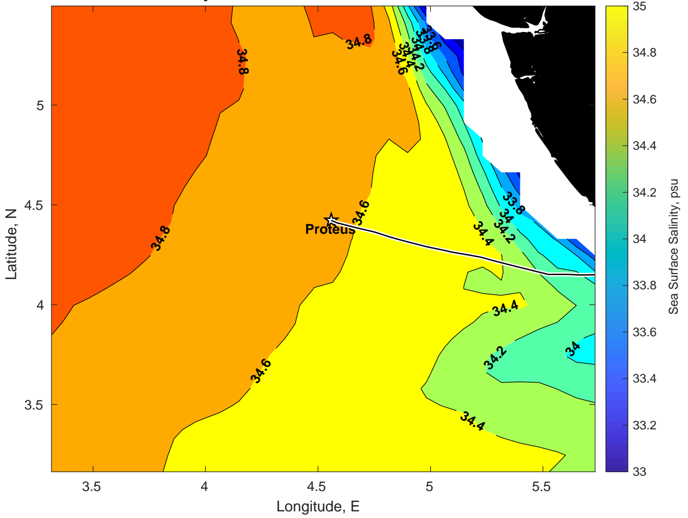
Surface Salinity for Proteus at 04-Feb-2025 00:00:00
