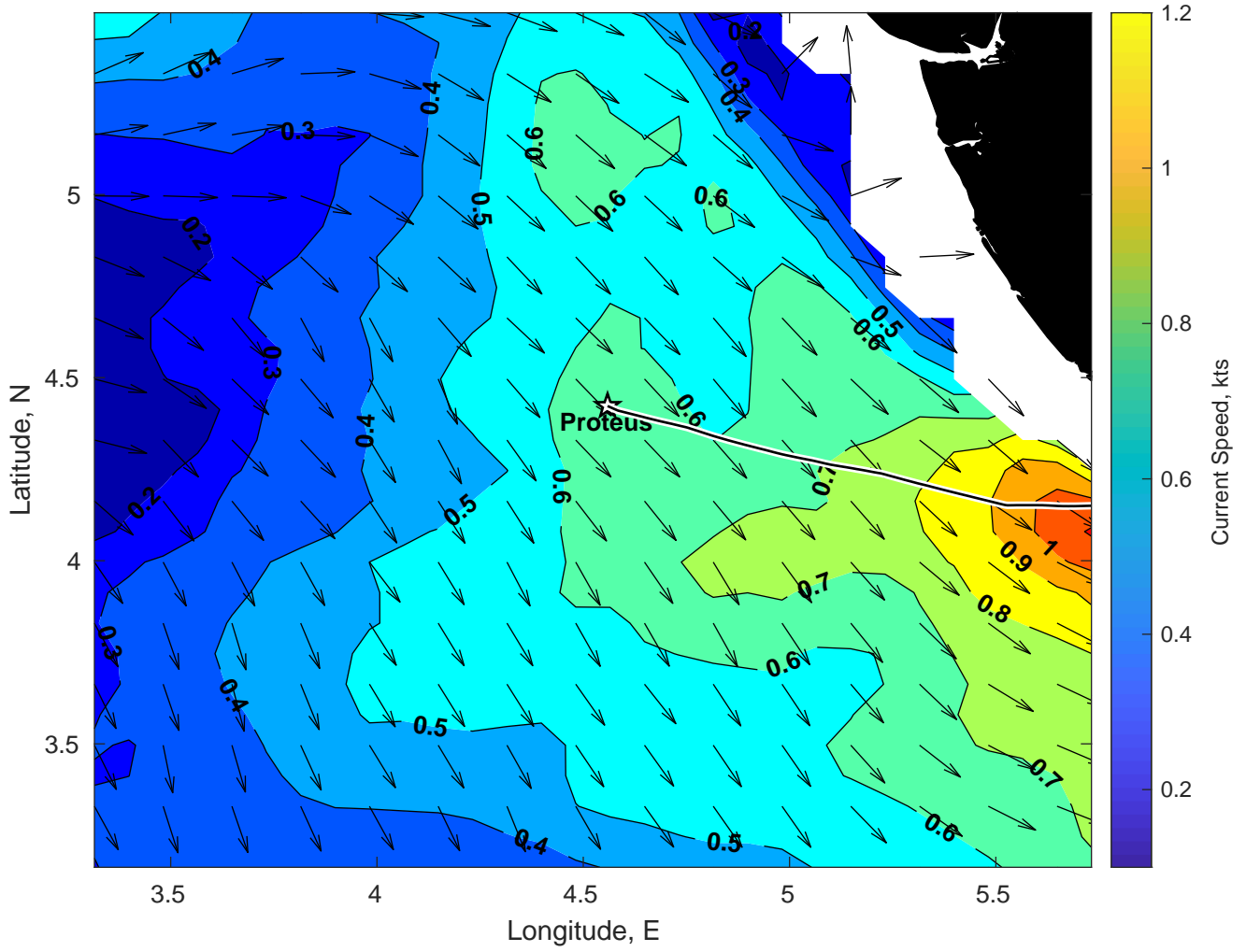
Surface Currents for Proteus at 04-Feb-2025 00:00:00
