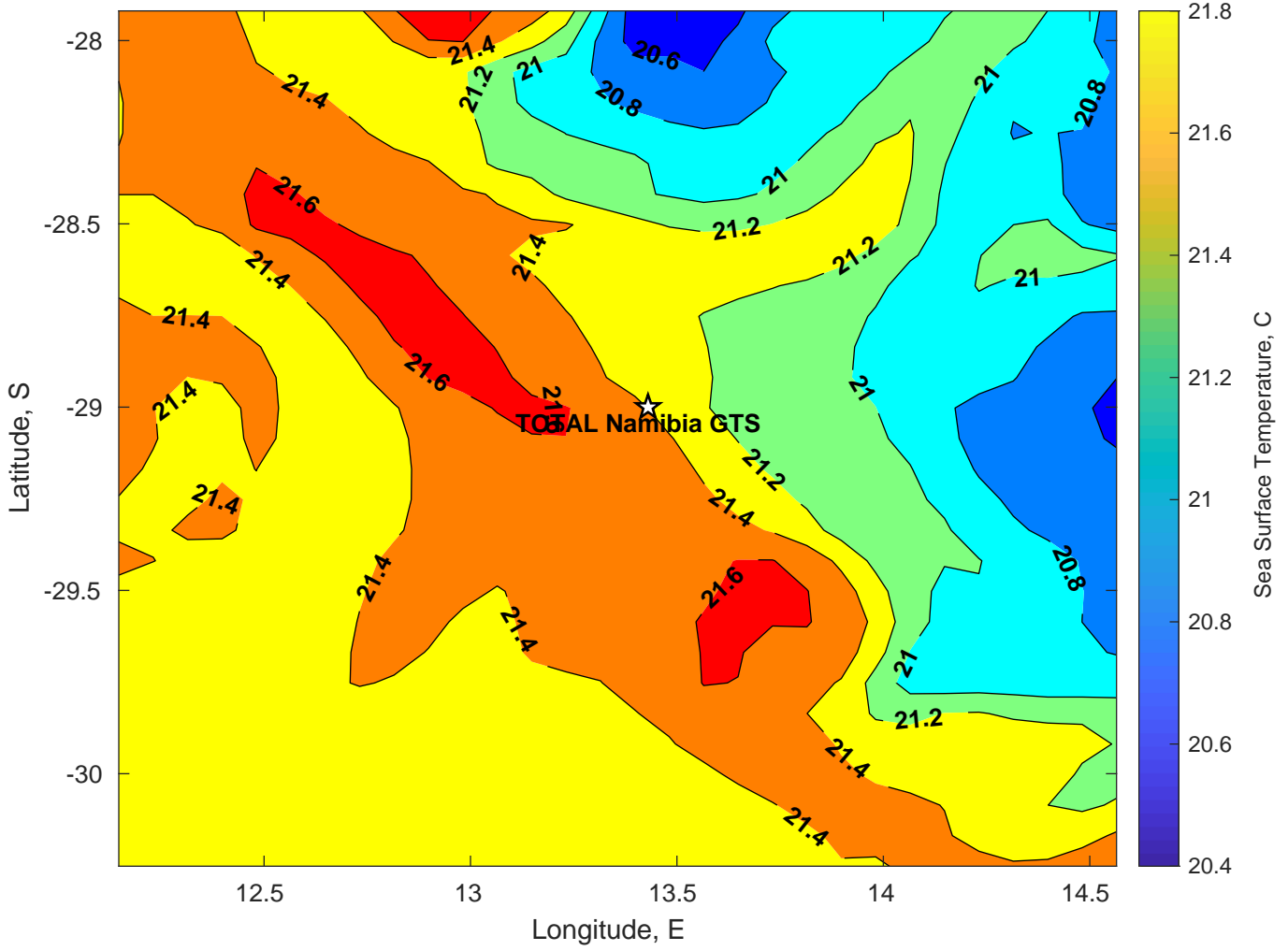
SST for TOTAL Namibia GTS at 04-Feb-2025 00:00:00
