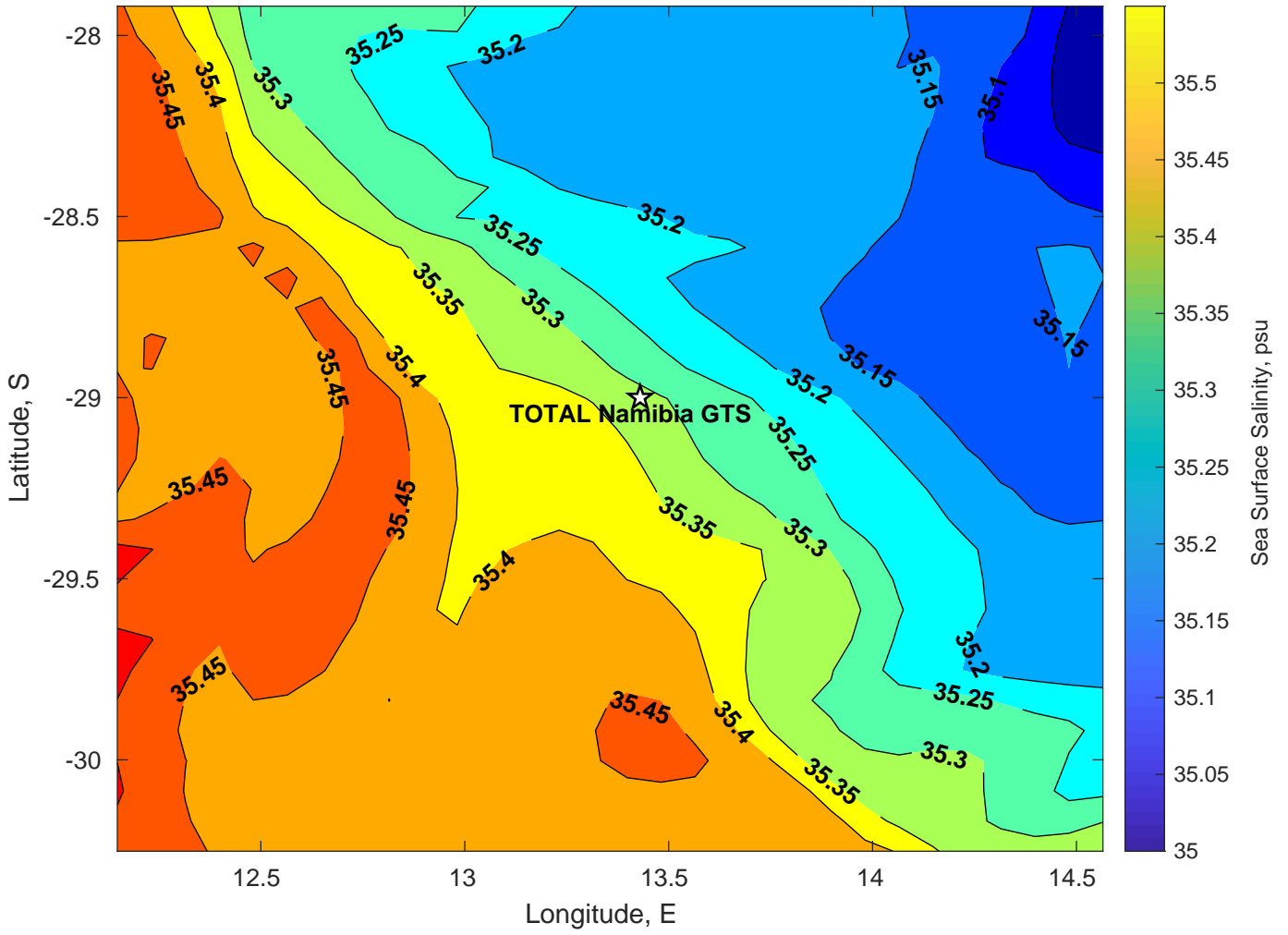
Surface Salinity for TOTAL Namibia GTS at 04-Feb-2025 00:00:00
