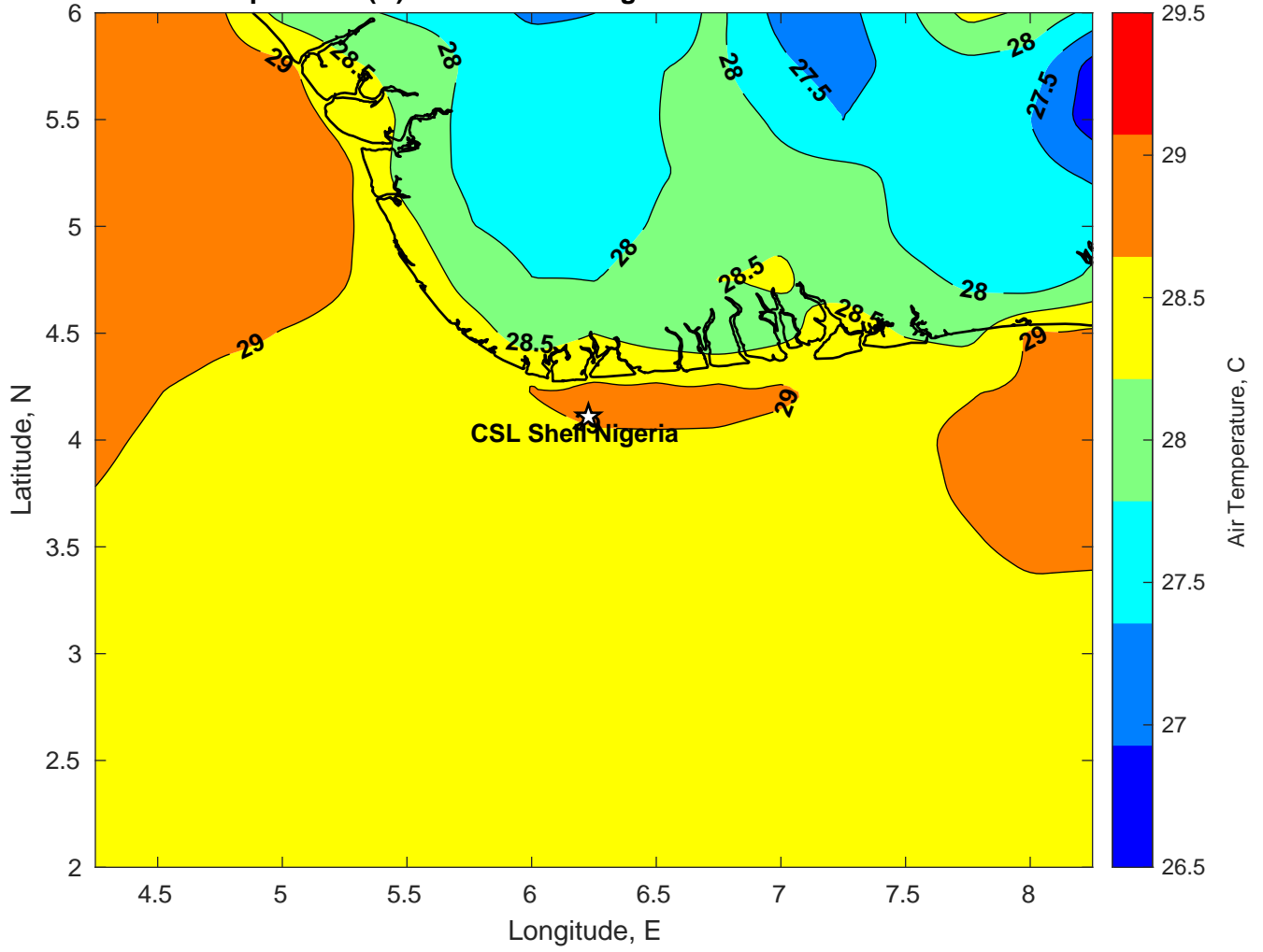
Air Temperature (C) for CSL Shell Nigeria at 05-Feb-2025
