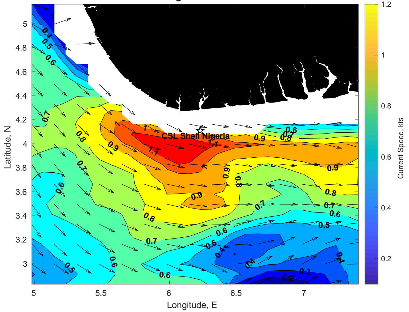
Surface Currents for CSL Shell Nigeria at 04-Feb-2025 00:00:00
