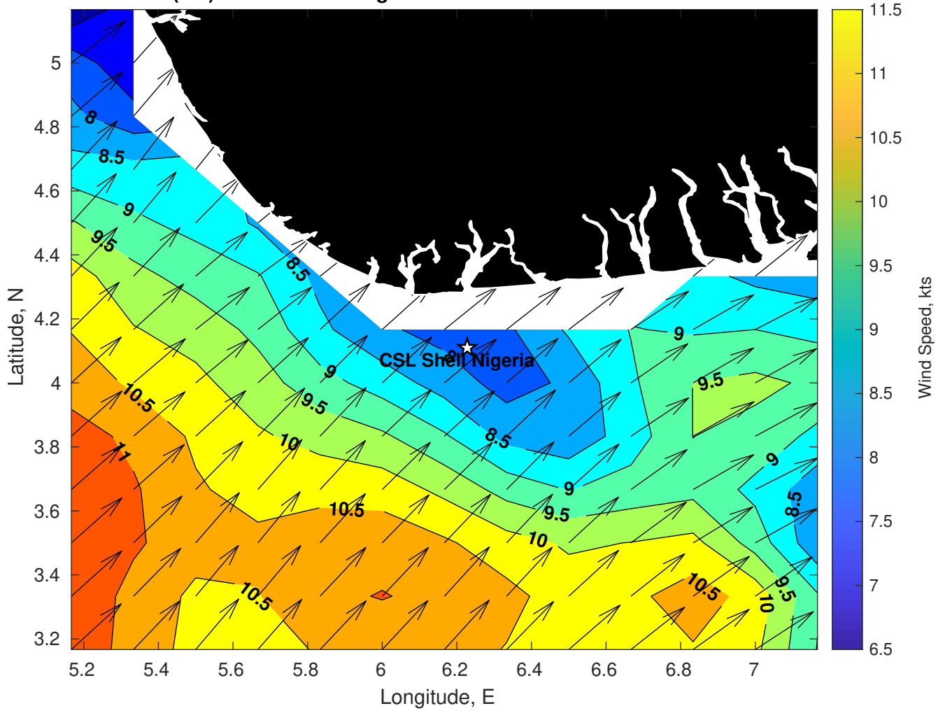
Winds (kts) for CSL Shell Nigeria at 05-Feb-2025 09:00:00
