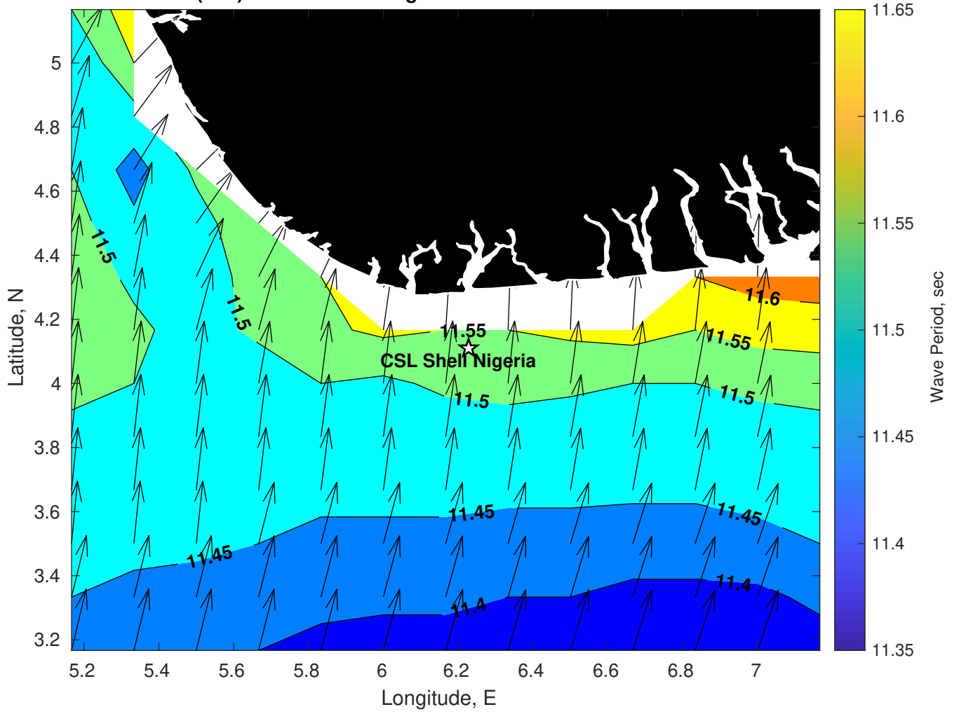
Wave Period (sec) for CSL Shell Nigeria at 05-Feb-2025 09:00:00
