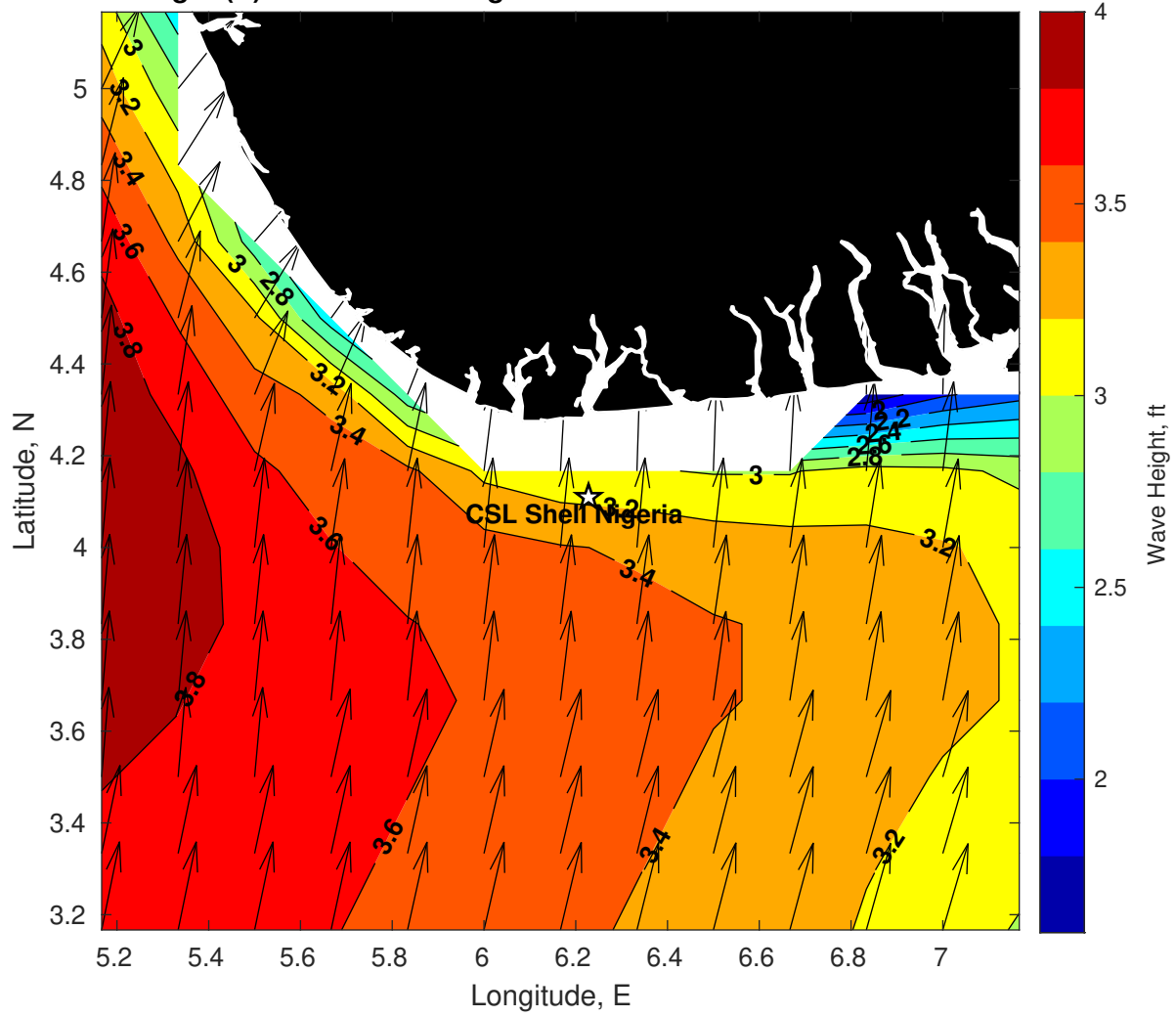
Wave Height (ft) for CSL Shell Nigeria at 05-Feb-2025 09:00:00
