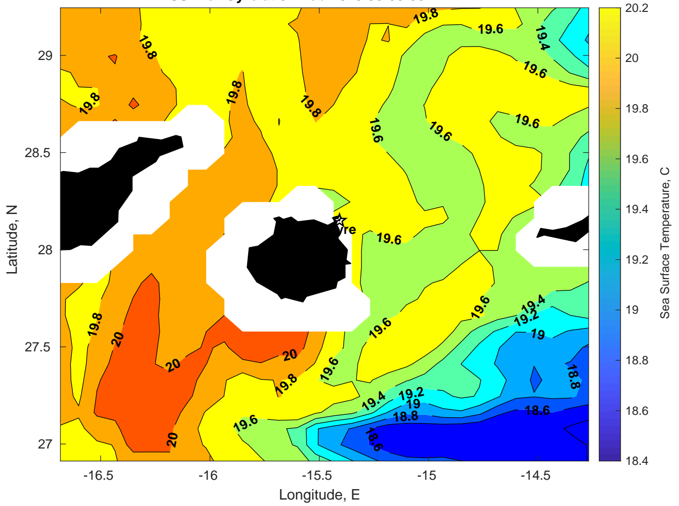
SST for Gyre at 04-Feb-2025 00:00:00
