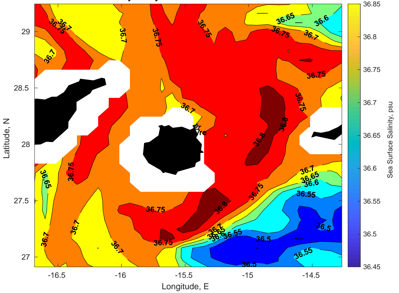
Surface Salinity for Gyre at 04-Feb-2025 00:00:00
