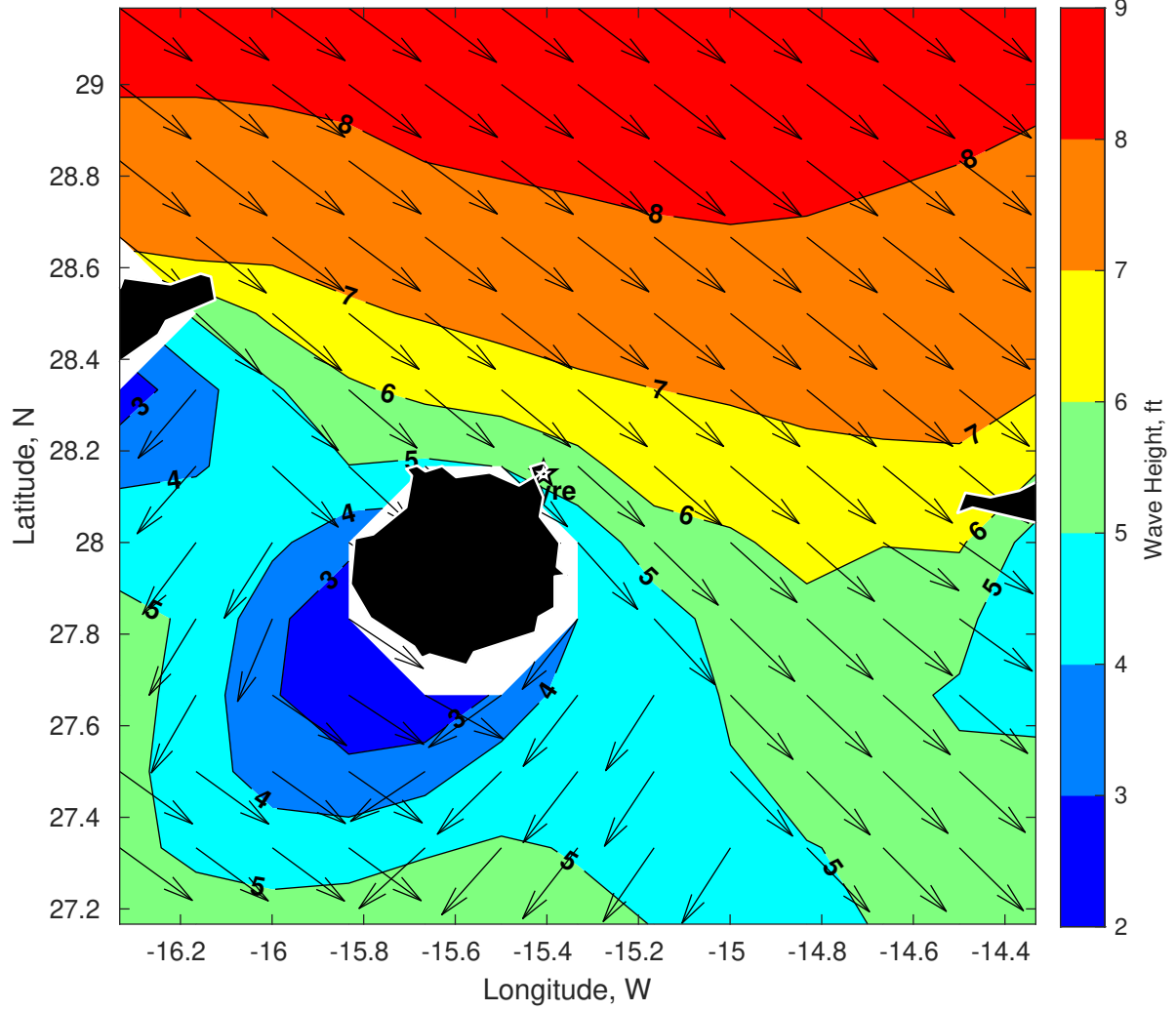
Wave Height (ft) for Gyre at 05-Feb-2025 09:00:00
