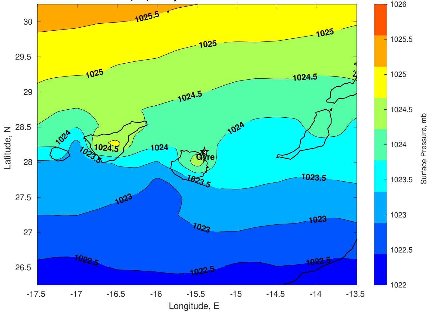
Surface Pressure (mb) for Gyre at 07-Feb-2025 00:00:00
