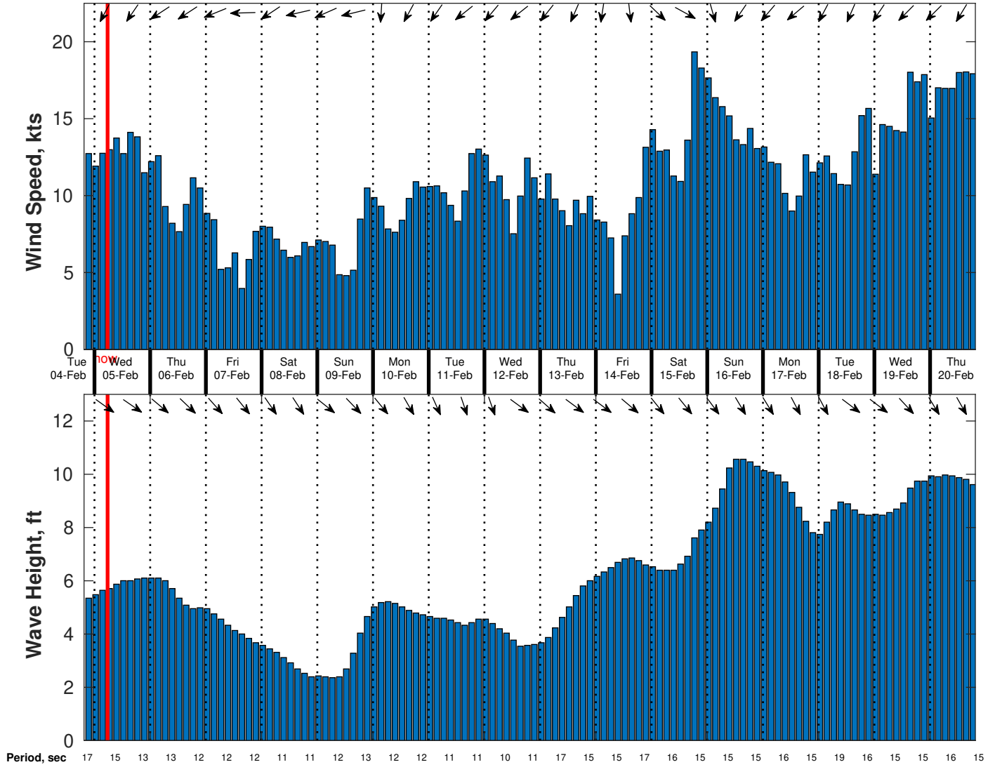
Wind & Wave Forecast for Gyre from 04-Feb-2025 20:00:00 to 20-Feb-2025 20:00:00
