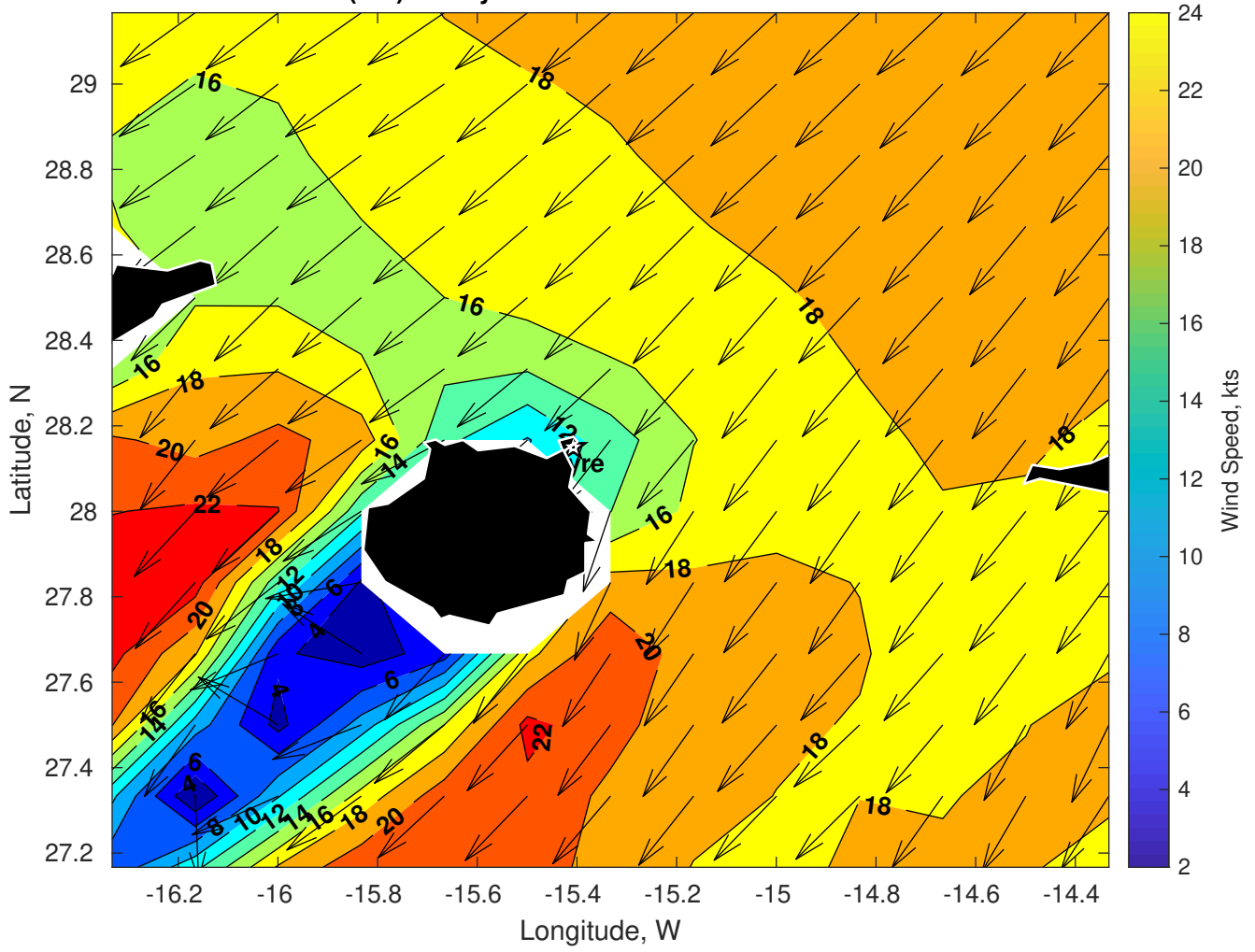
Winds (kts) for Gyre at 05-Feb-2025 09:00:00
