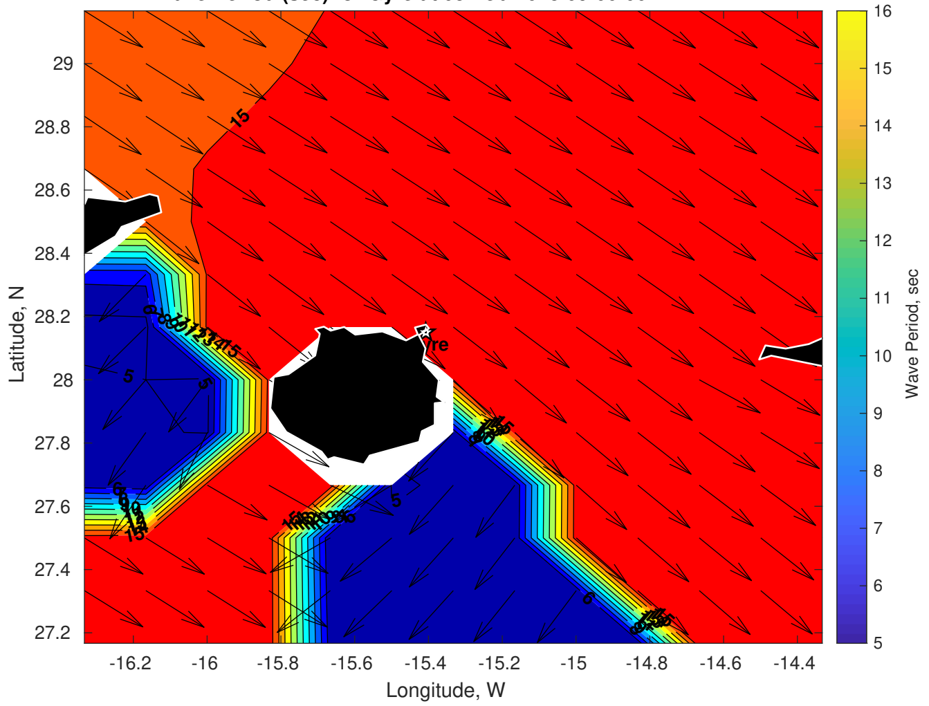
Wave Period (sec) for Gyre at 05-Feb-2025 09:00:00
