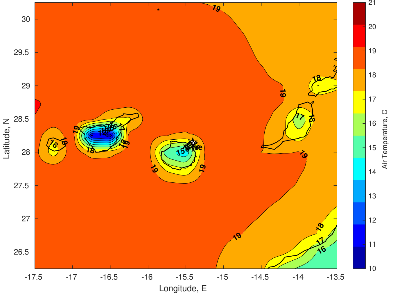
Air Temperature (C) for Gyre at 05-Feb-2025
