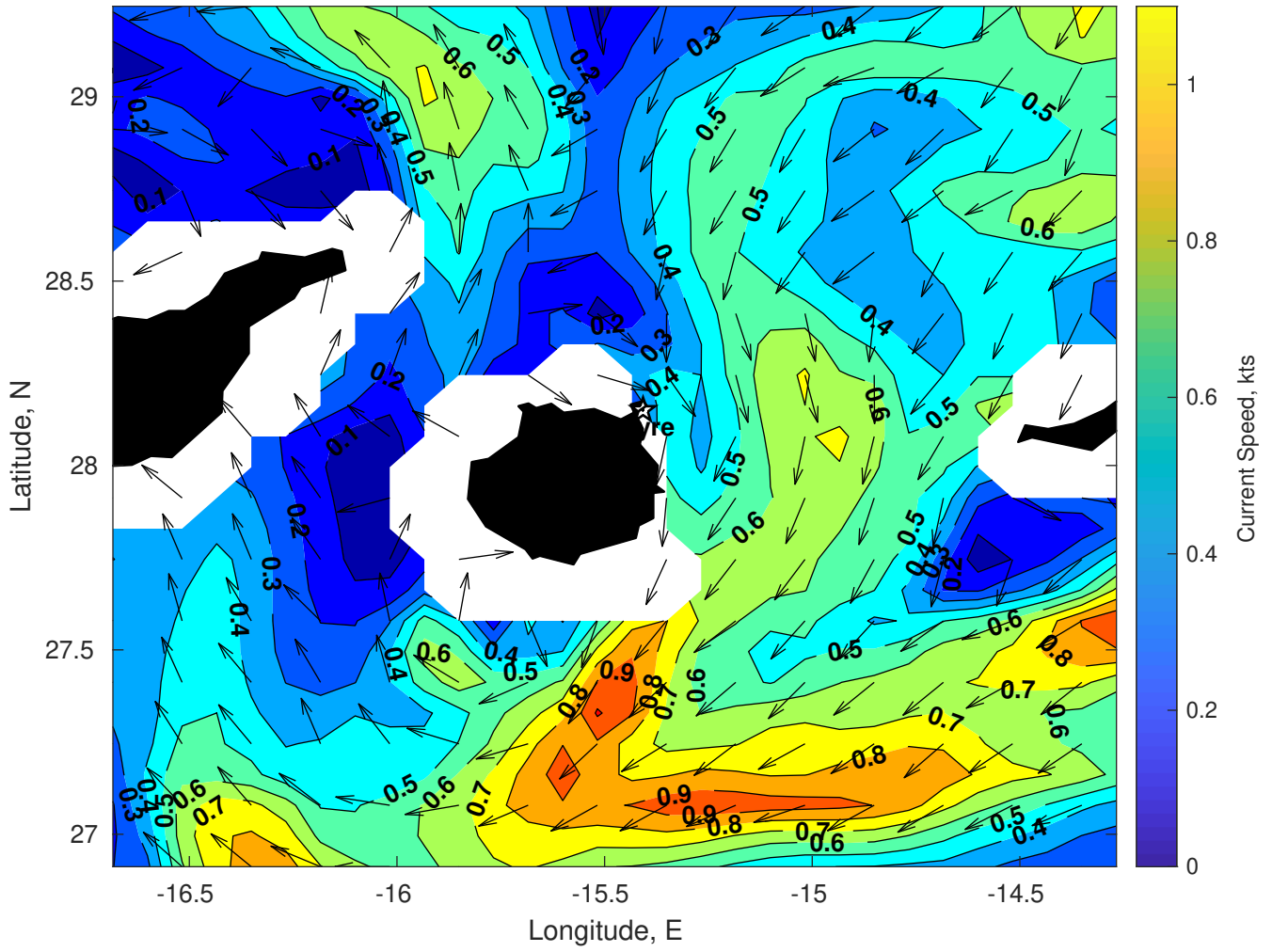
Surface Currents for Gyre at 04-Feb-2025 00:00:00
