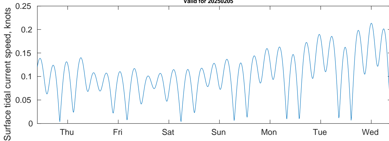
Tidal Currents and Heights for Gyre at 20250205
