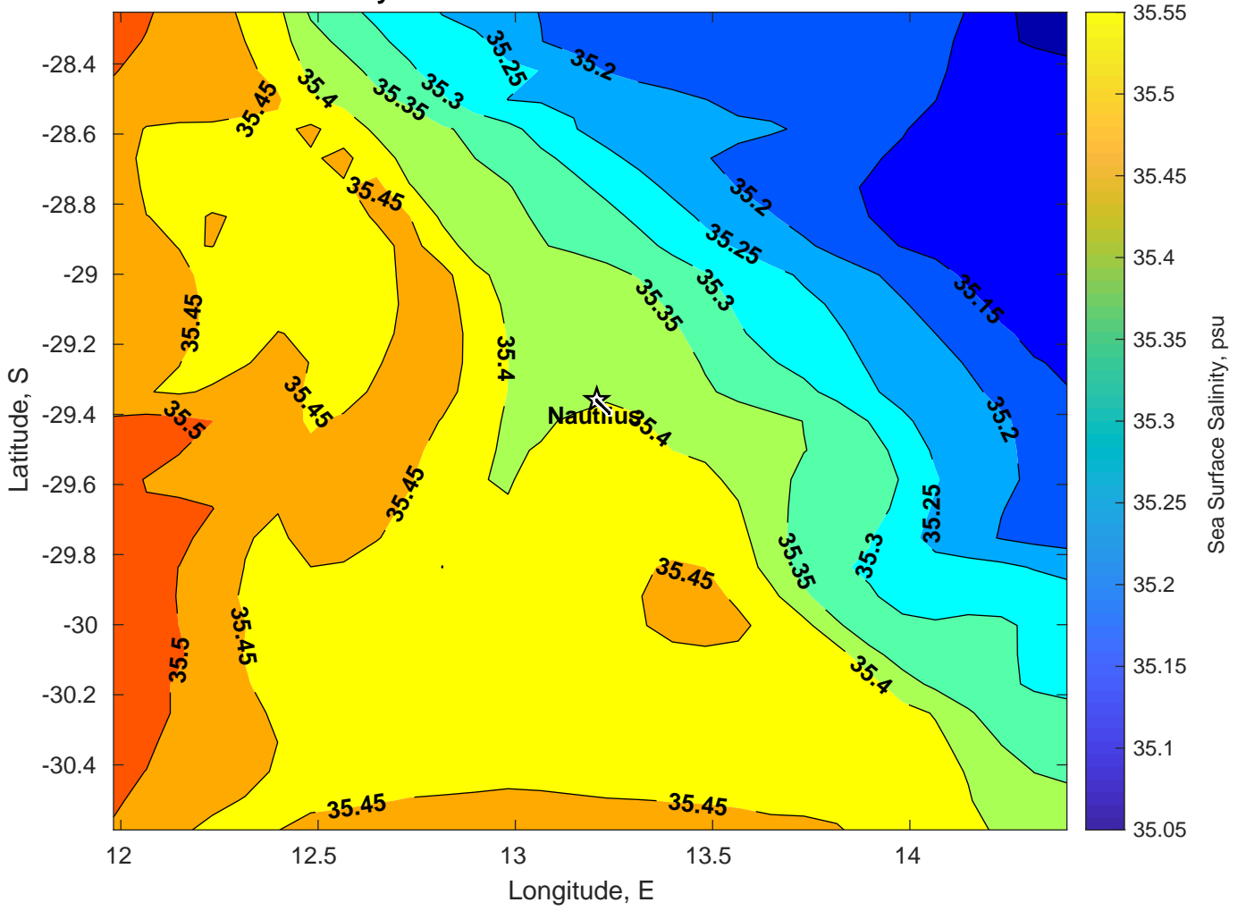
Surface Salinity for Nautilus at 04-Feb-2025 00:00:00
