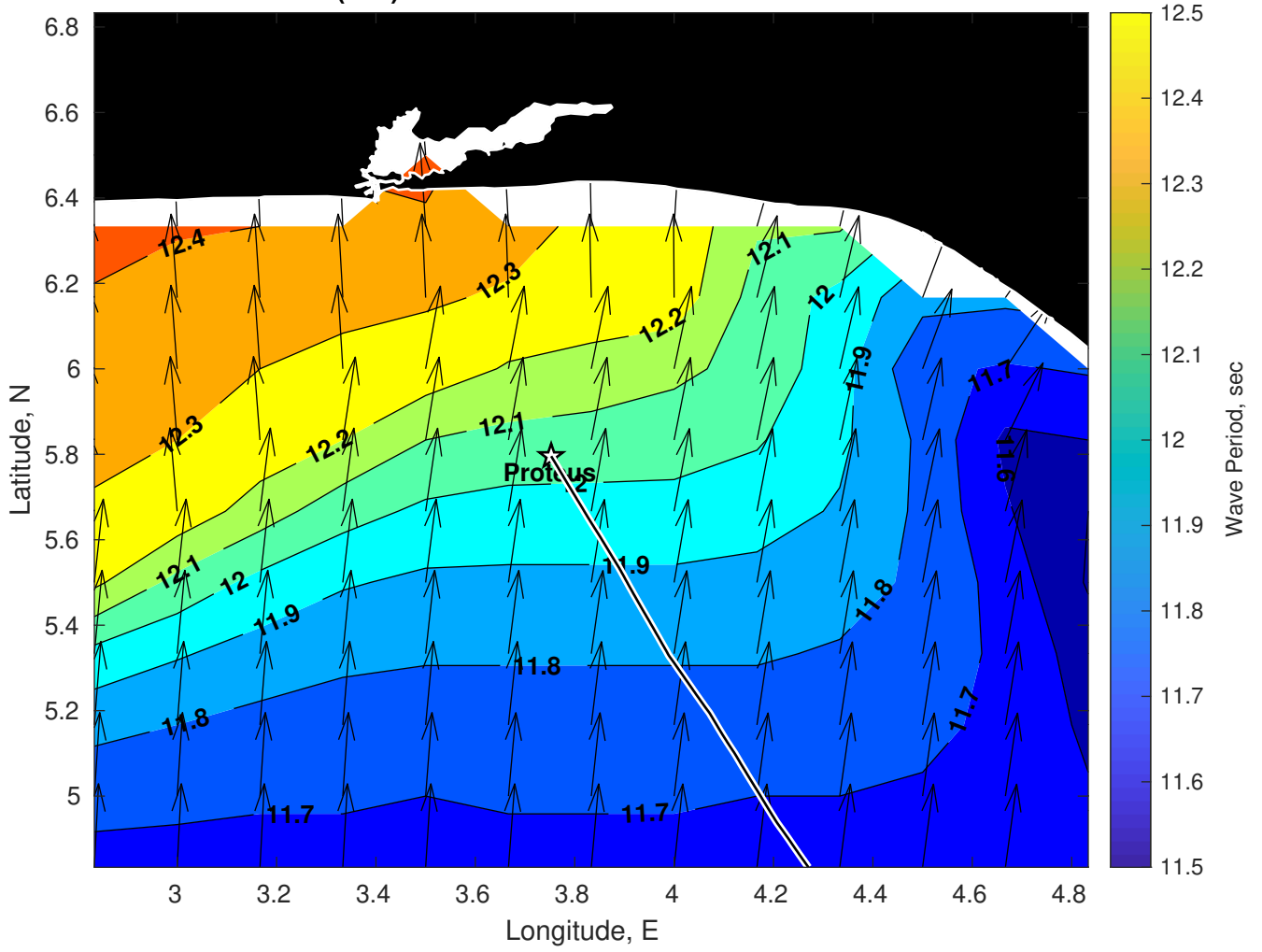
Wave Period (sec) for Proteus at 05-Feb-2025 09:00:00
