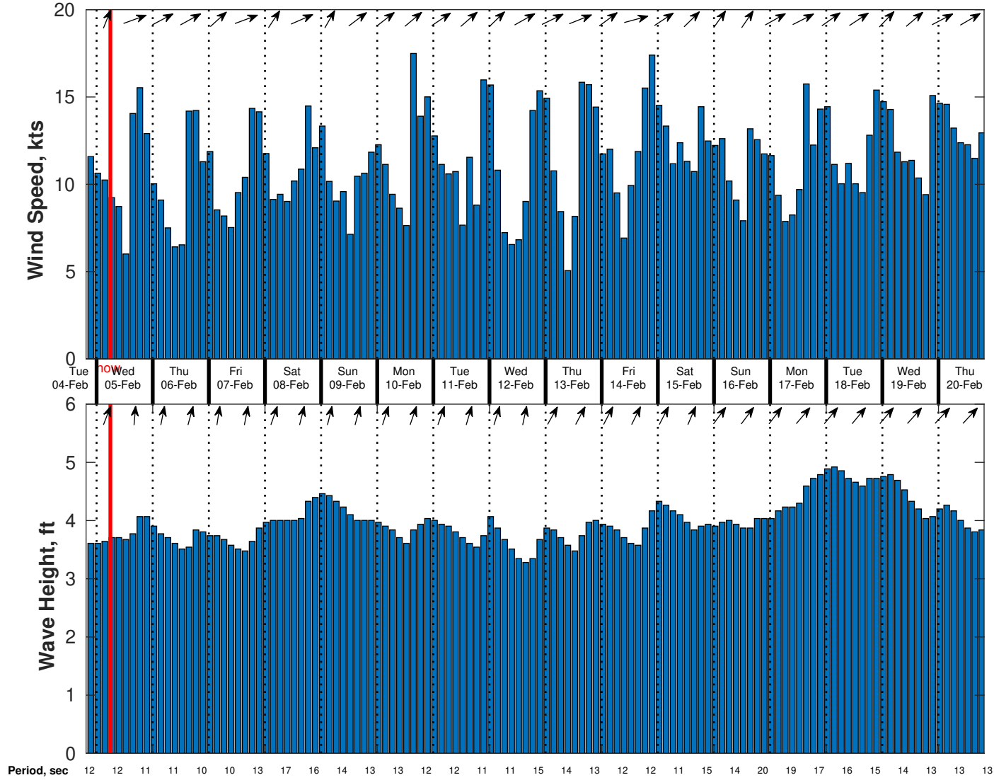
Wind & Wave Forecast for Proteus from 04-Feb-2025 20:00:00 to 20-Feb-2025 20:00:00
