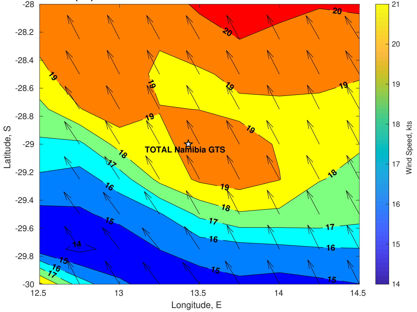
Winds (kts) for TOTAL Namibia GTS at 05-Feb-2025 09:00:00
