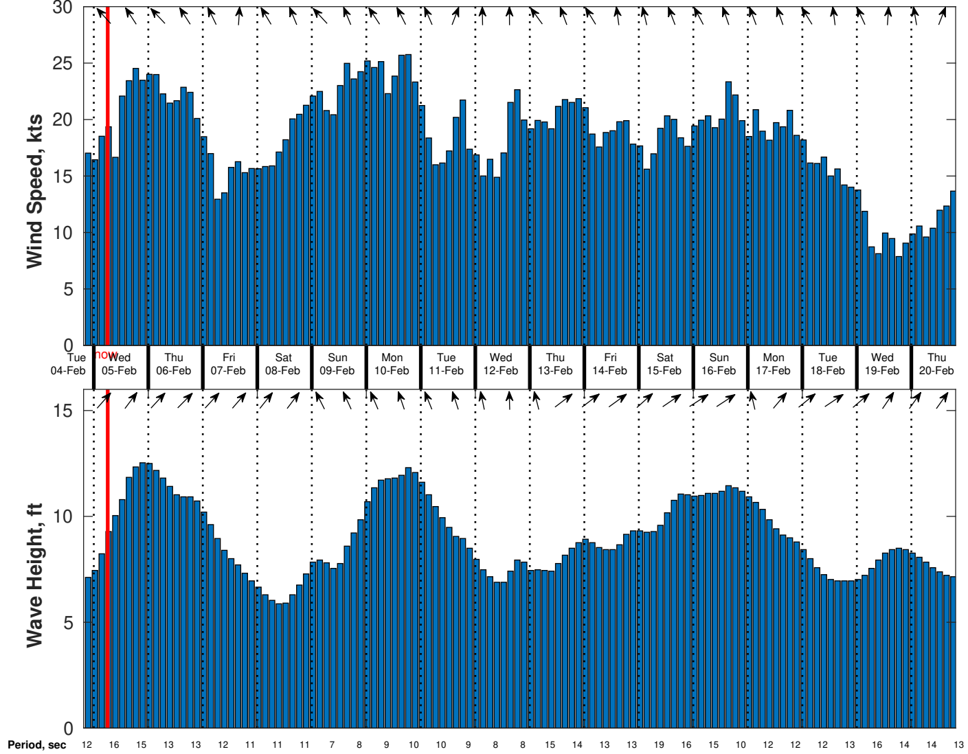
Wind & Wave Forecast for TOTAL Namibia GTS from 04-Feb-2025 20:00:00 to 20-Feb-2025 20:00:00
