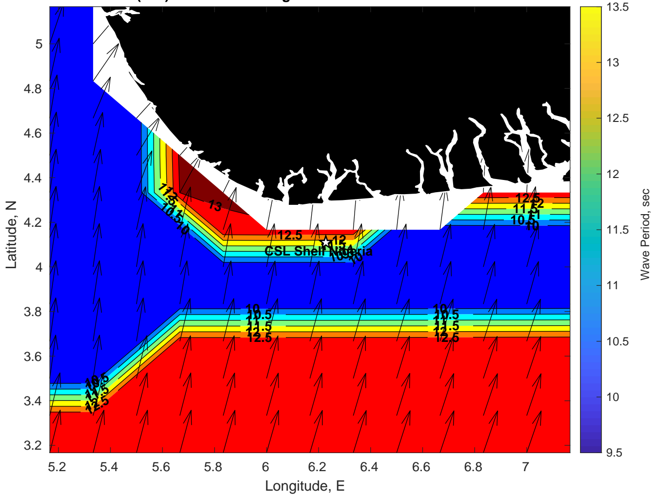
Wave Period (sec) for CSL Shell Nigeria at 07-Feb-2025 09:00:00
