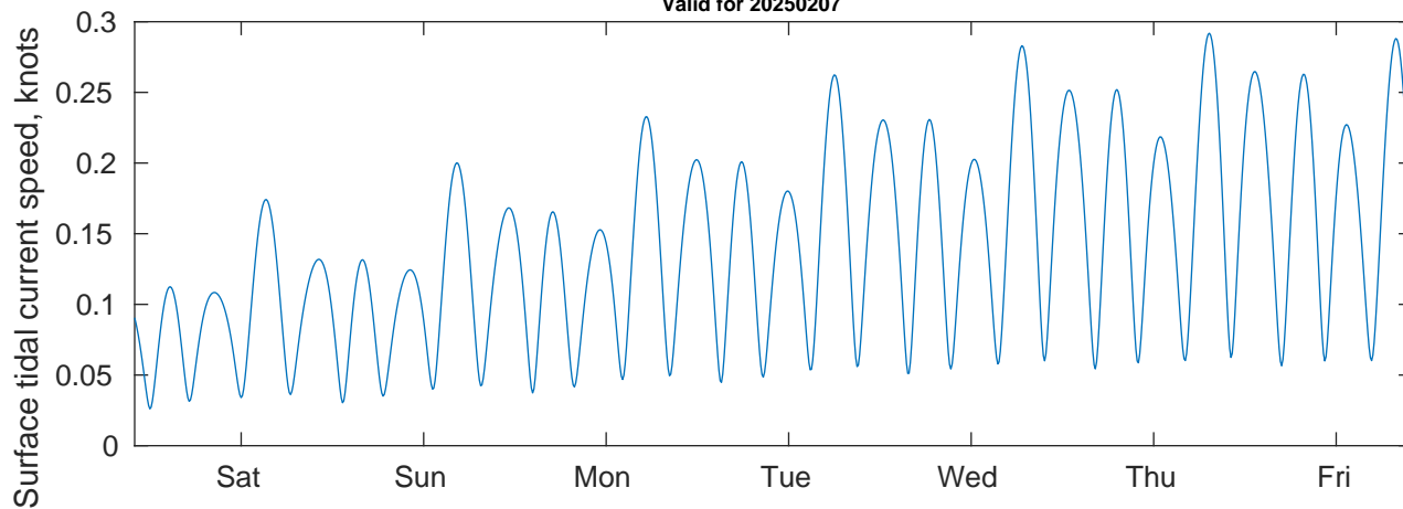
Tidal Currents and Heights for CSL Shell Nigeria at 20250207
