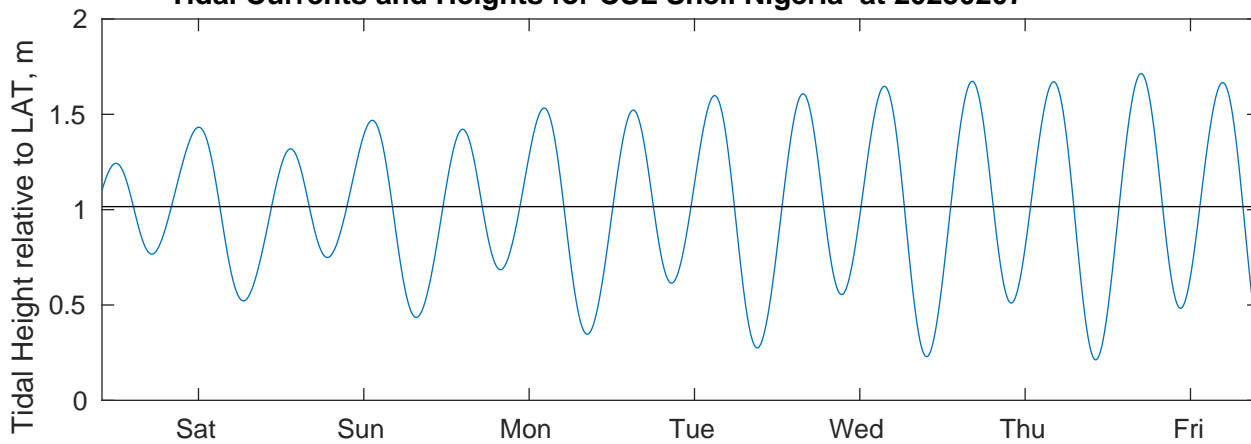
Tidal Currents and Heights for CSL Shell Nigeria at 20250207
