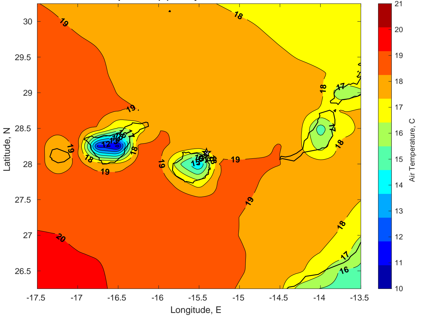
Air Temperature (C) for Gyre at 07-Feb-2025
