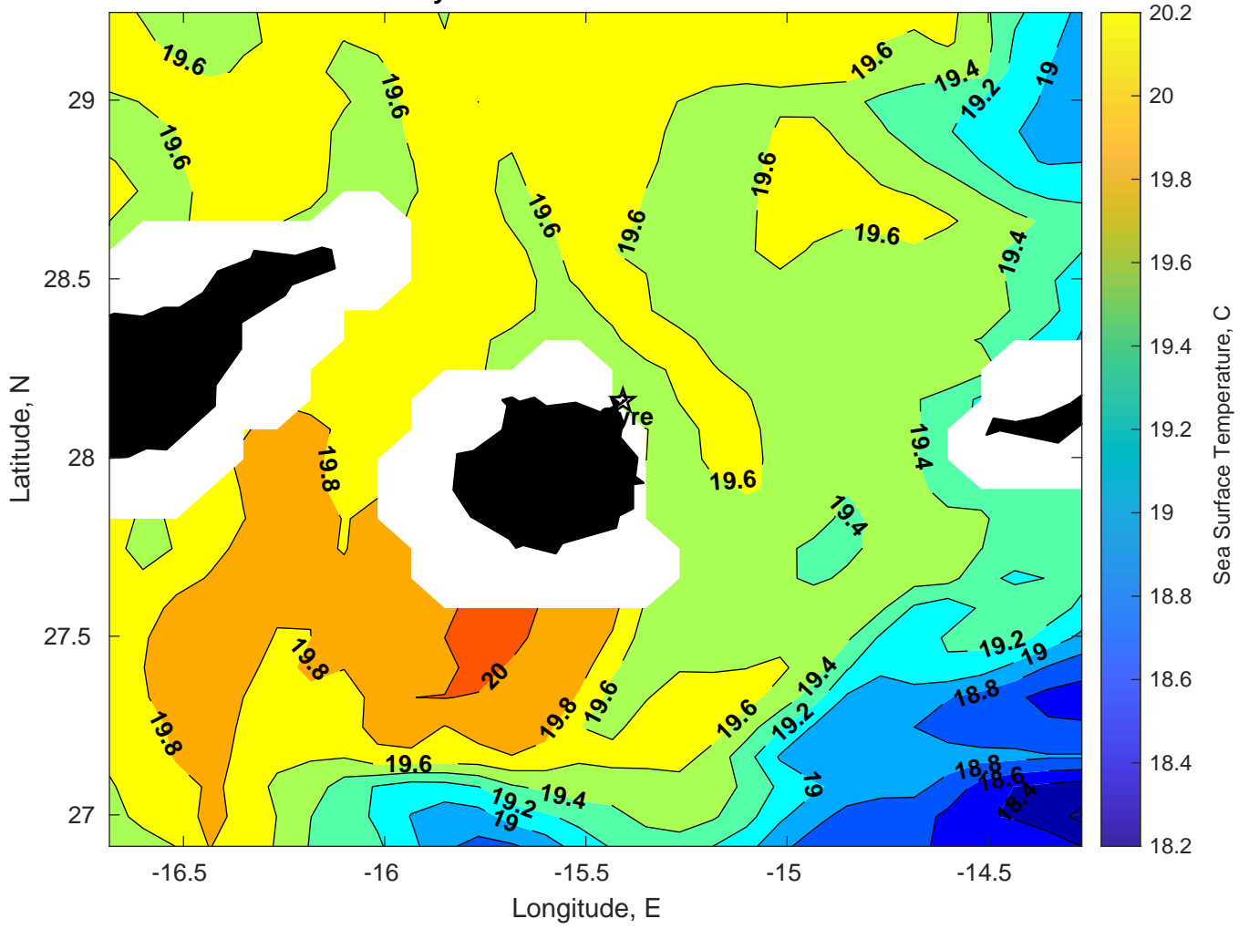
SST for Gyre at 06-Feb-2025 00:00:00
