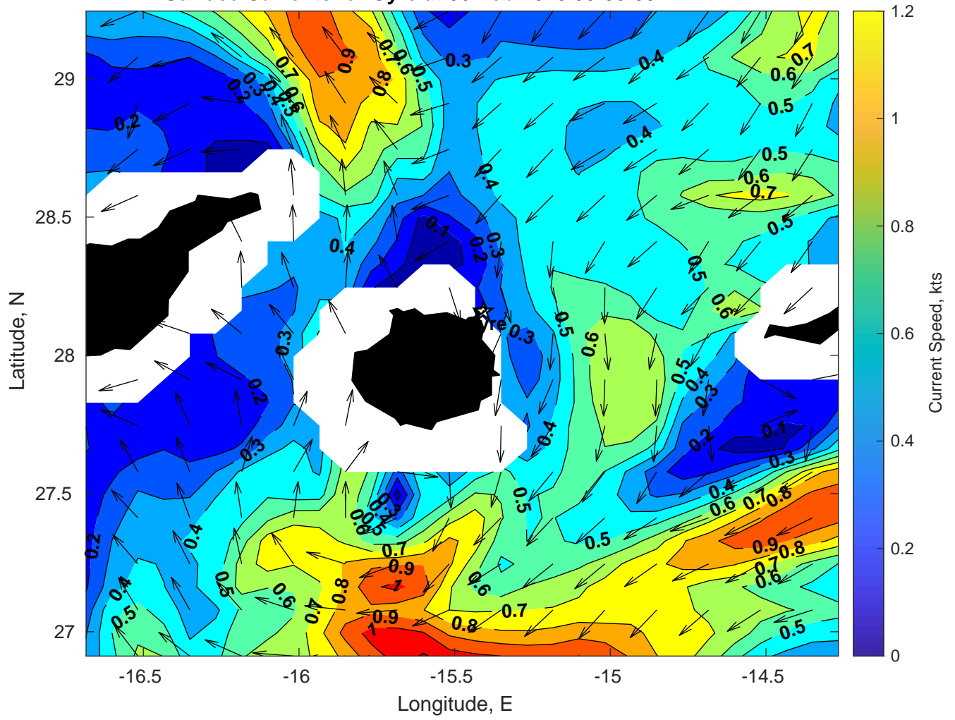
Surface Currents for Gyre at 06-Feb-2025 00:00:00
