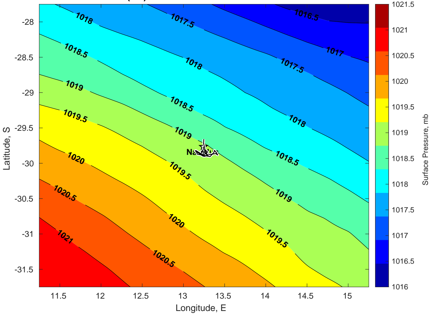
Surface Pressure (mb) for Nautilus at 09-Feb-2025 00:00:00
