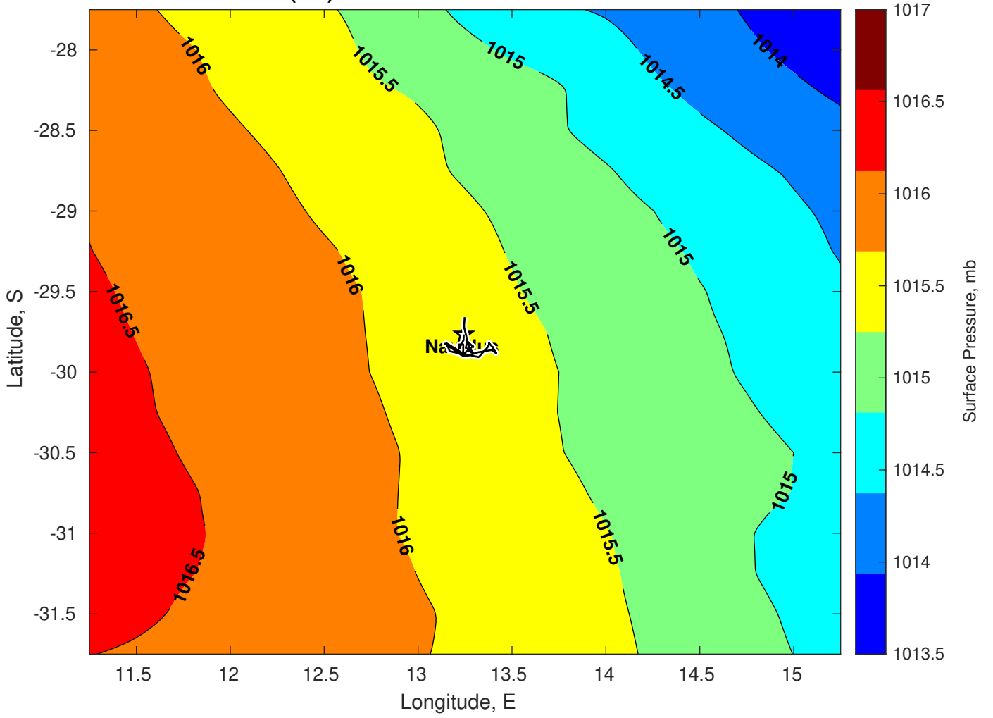
Surface Pressure (mb) for Nautilus at 08-Feb-2025 00:00:00
