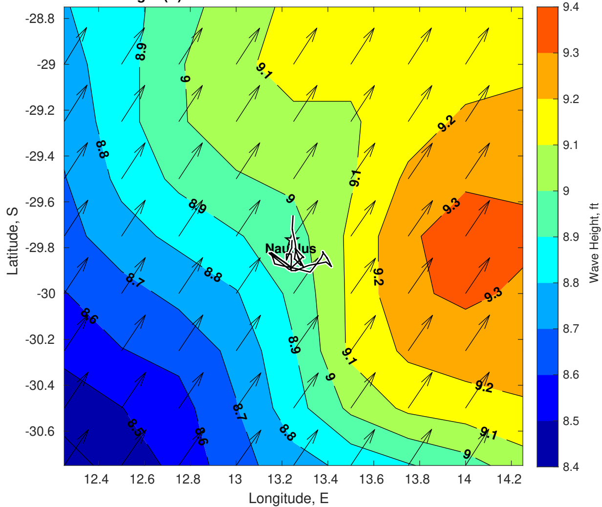
Wave Height (ft) for Nautilus at 07-Feb-2025 09:00:00
