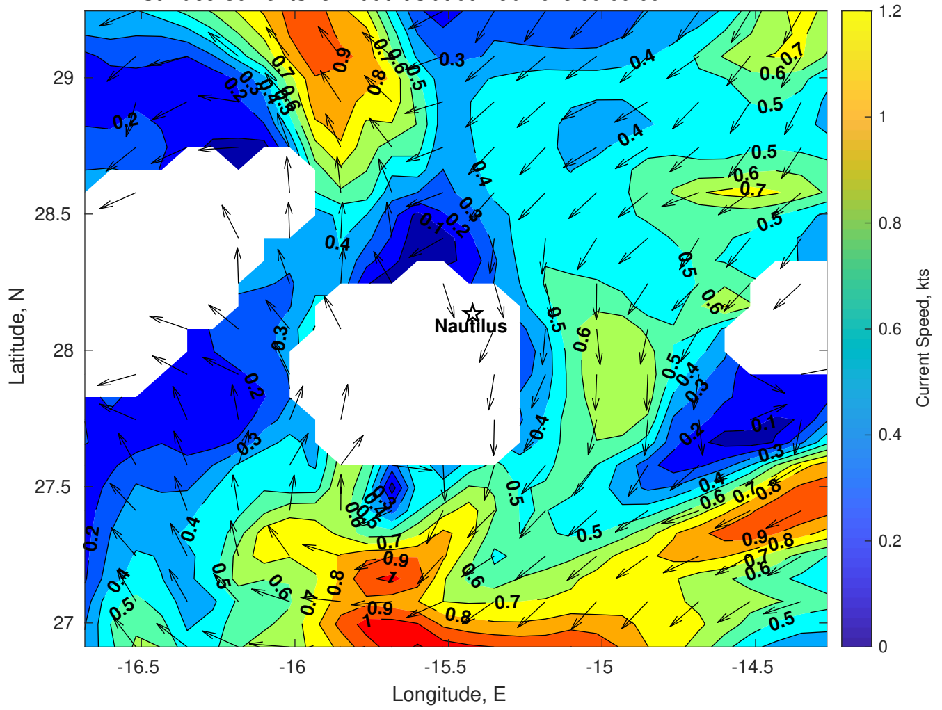
Surface Currents for Nautilus at 06-Feb-2025 00:00:00
