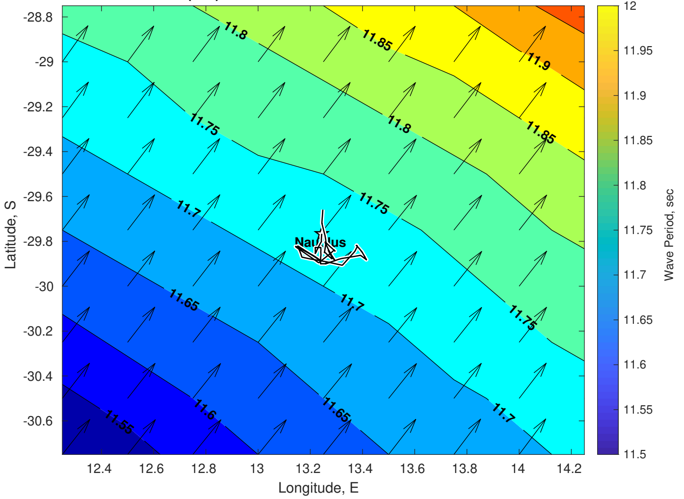
Wave Period (sec) for Nautilus at 07-Feb-2025 09:00:00
