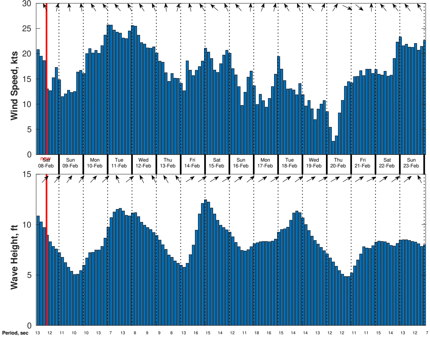
Wind & Wave Forecast for Nautilus from 07-Feb-2025 02:00:00 to 23-Feb-2025 02:00:00
