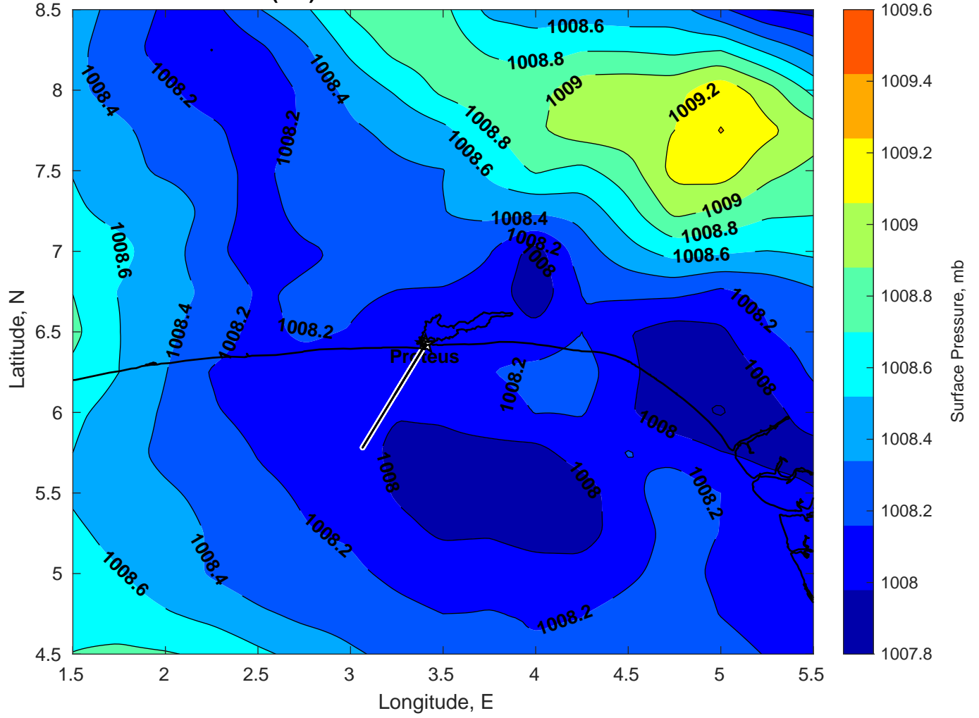
Surface Pressure (mb) for Proteus at 07-Feb-2025 00:00:00
