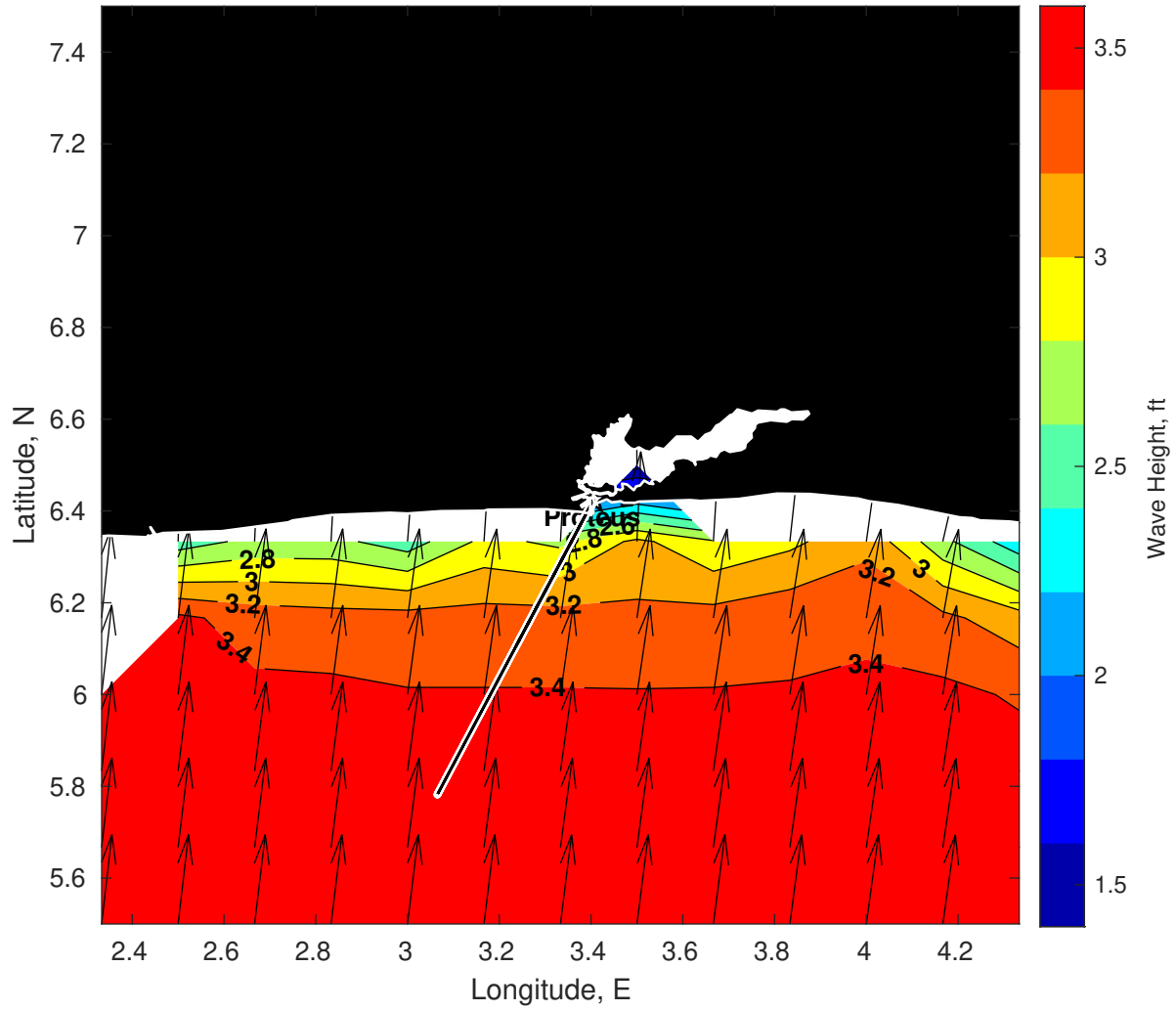
Wave Height (ft) for Proteus at 07-Feb-2025 09:00:00
