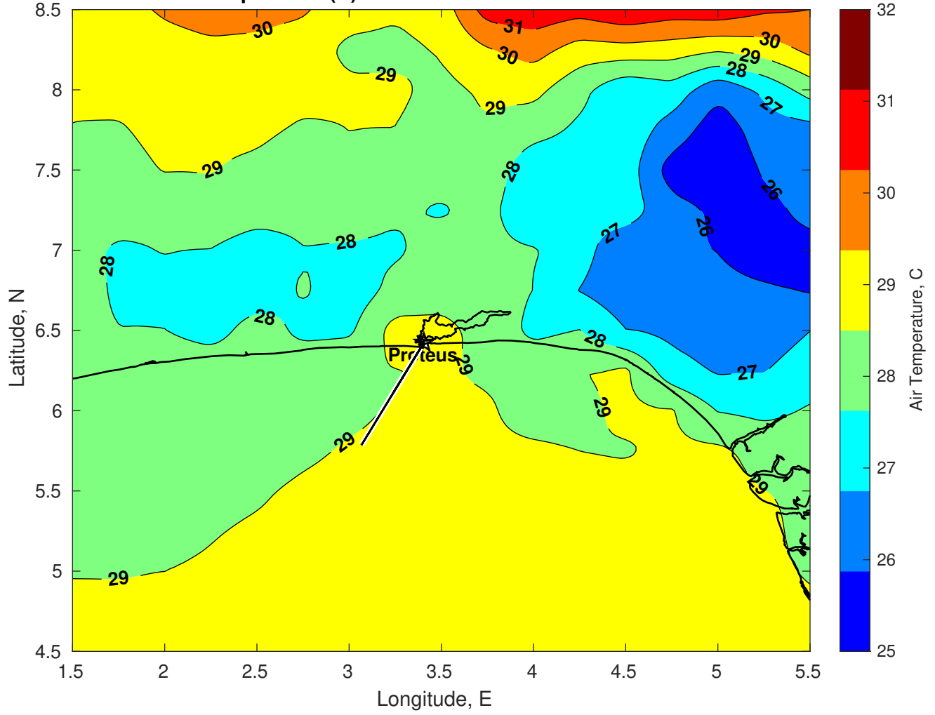
Air Temperature (C) for Proteus at 07-Feb-2025
