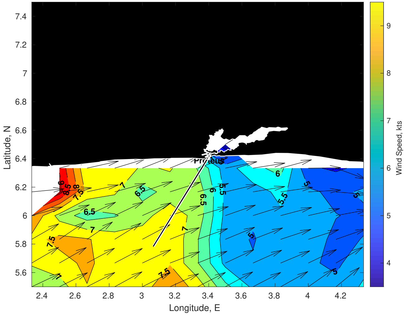
Winds (kts) for Proteus at 07-Feb-2025 09:00:00
