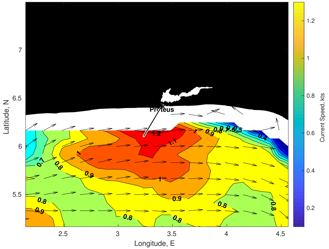
Surface Currents for Proteus at 06-Feb-2025 00:00:00
