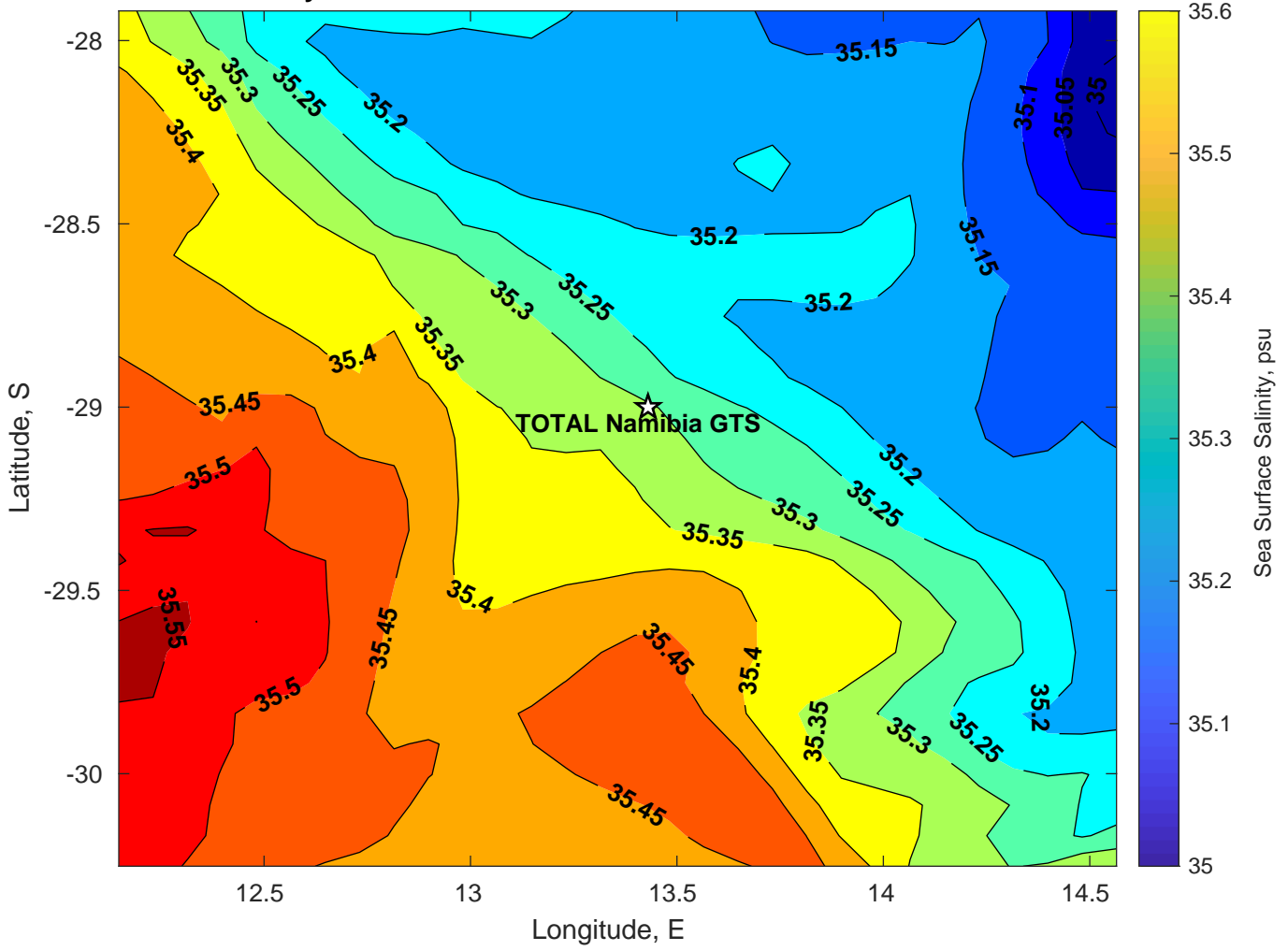
Surface Salinity for TOTAL Namibia GTS at 06-Feb-2025 00:00:00
