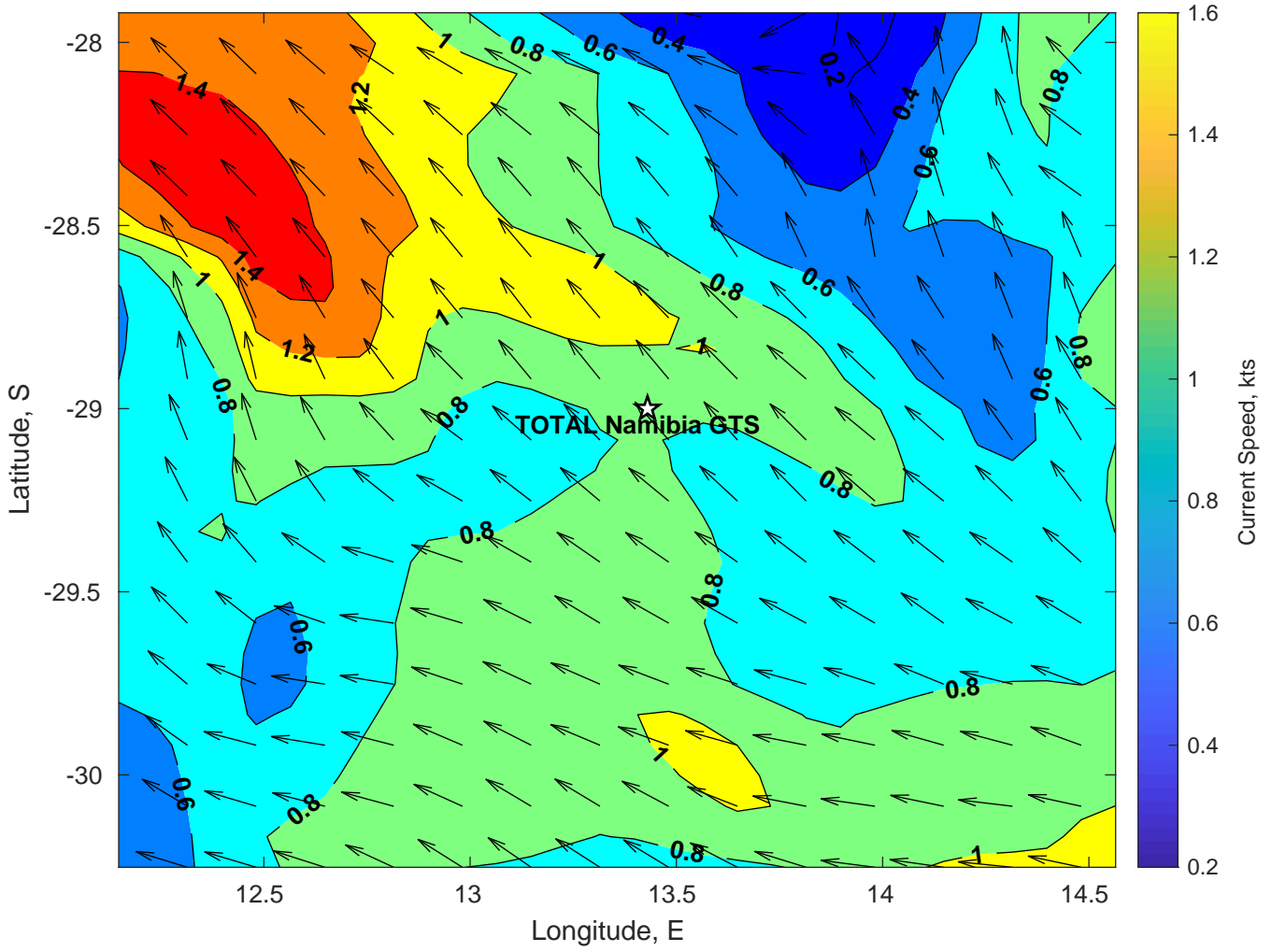
Surface Currents for TOTAL Namibia GTS at 06-Feb-2025 00:00:00
