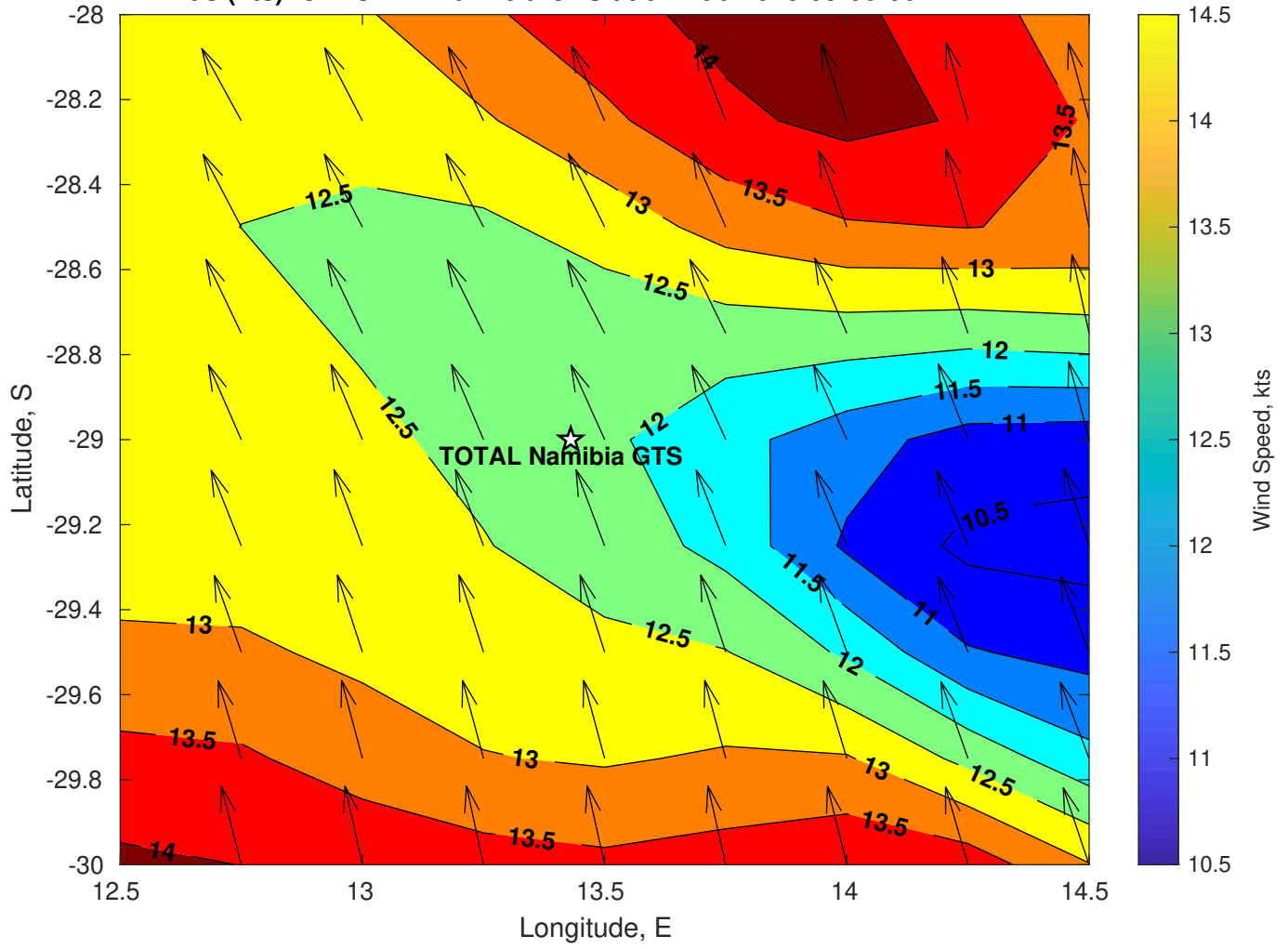
Winds (kts) for TOTAL Namibia GTS at 07-Feb-2025 09:00:00
