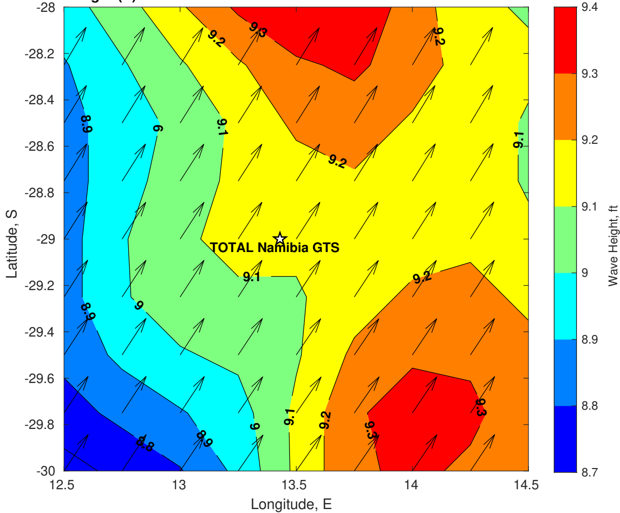
Wave Height (ft) for TOTAL Namibia GTS at 07-Feb-2025 09:00:00
