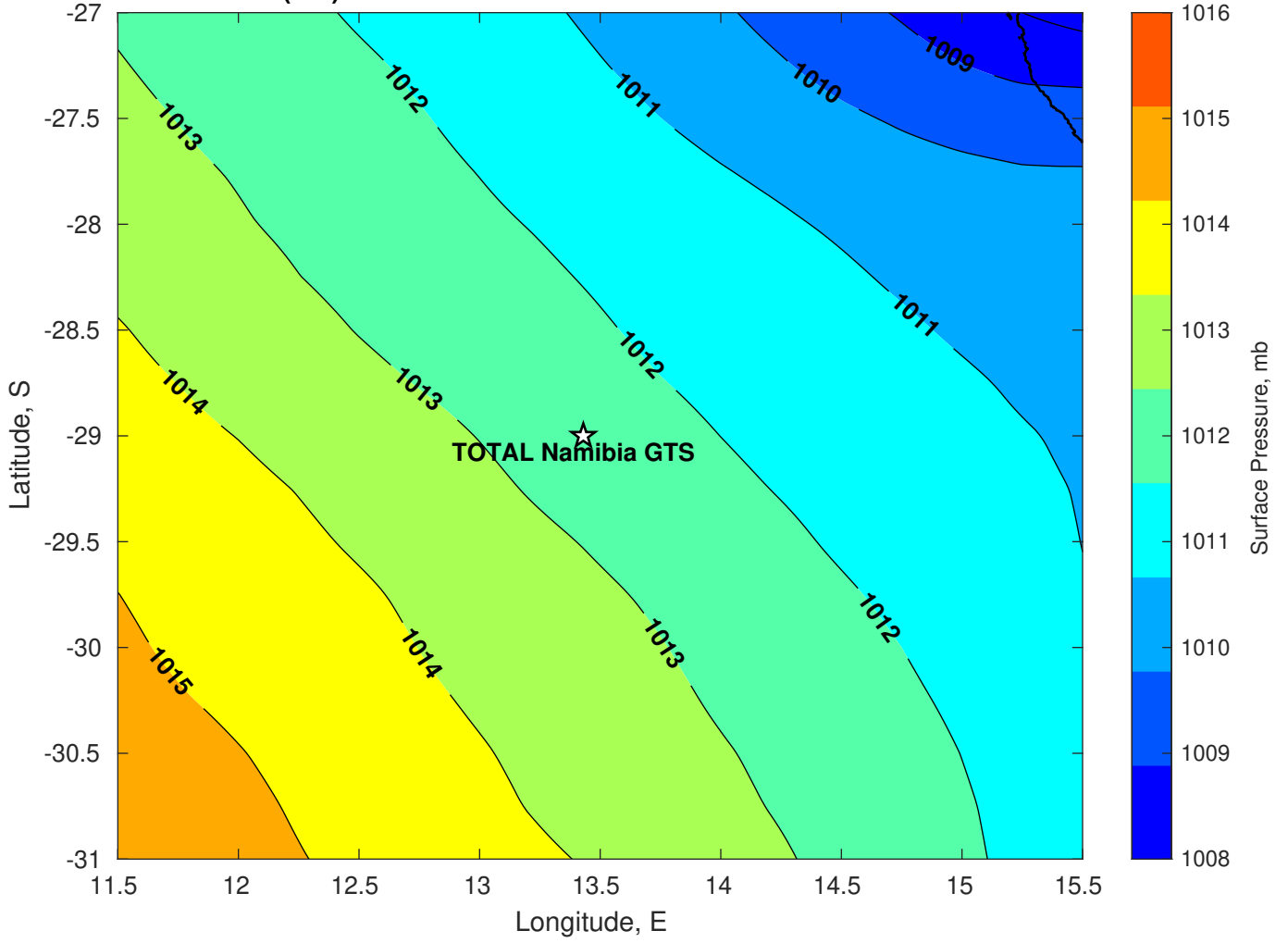
Surface Pressure (mb) for TOTAL Namibia GTS at 07-Feb-2025 00:00:00
