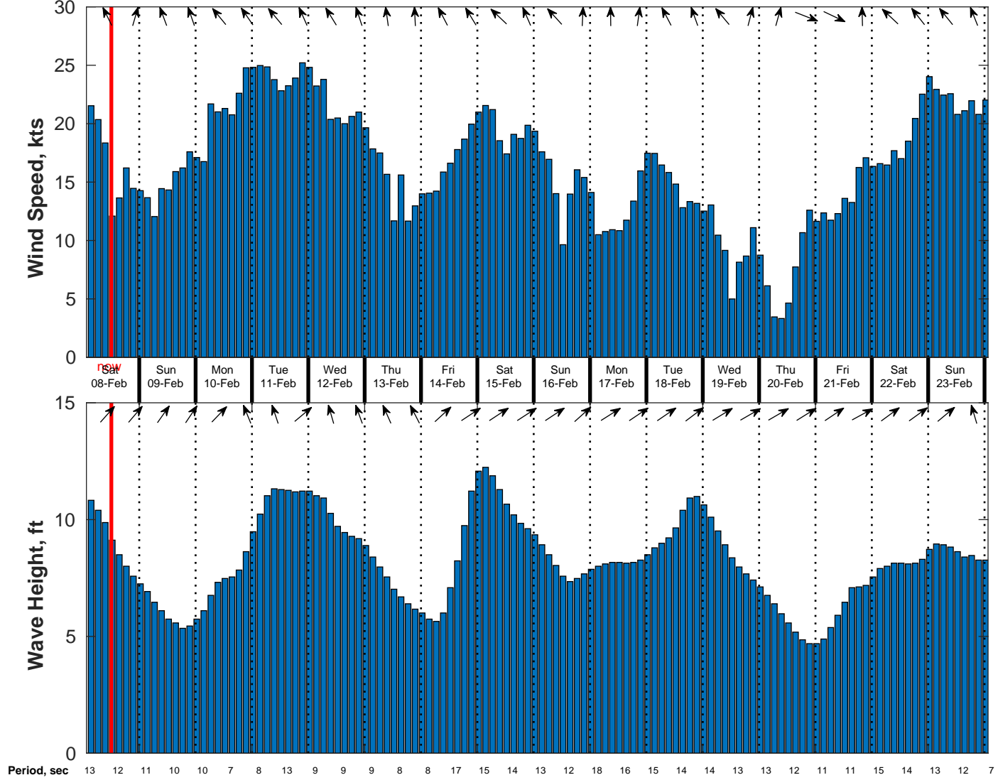
Wind & Wave Forecast for TOTAL Namibia GTS from 07-Feb-2025 02:00:00 to 23-Feb-2025 02:00:00
