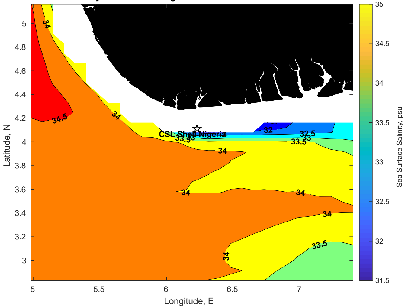
Surface Salinity for CSL Shell Nigeria at 07-Feb-2025 00:00:00
