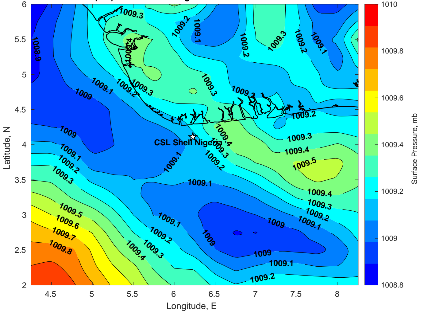
Surface Pressure (mb) for CSL Shell Nigeria at 08-Feb-2025 00:00:00
