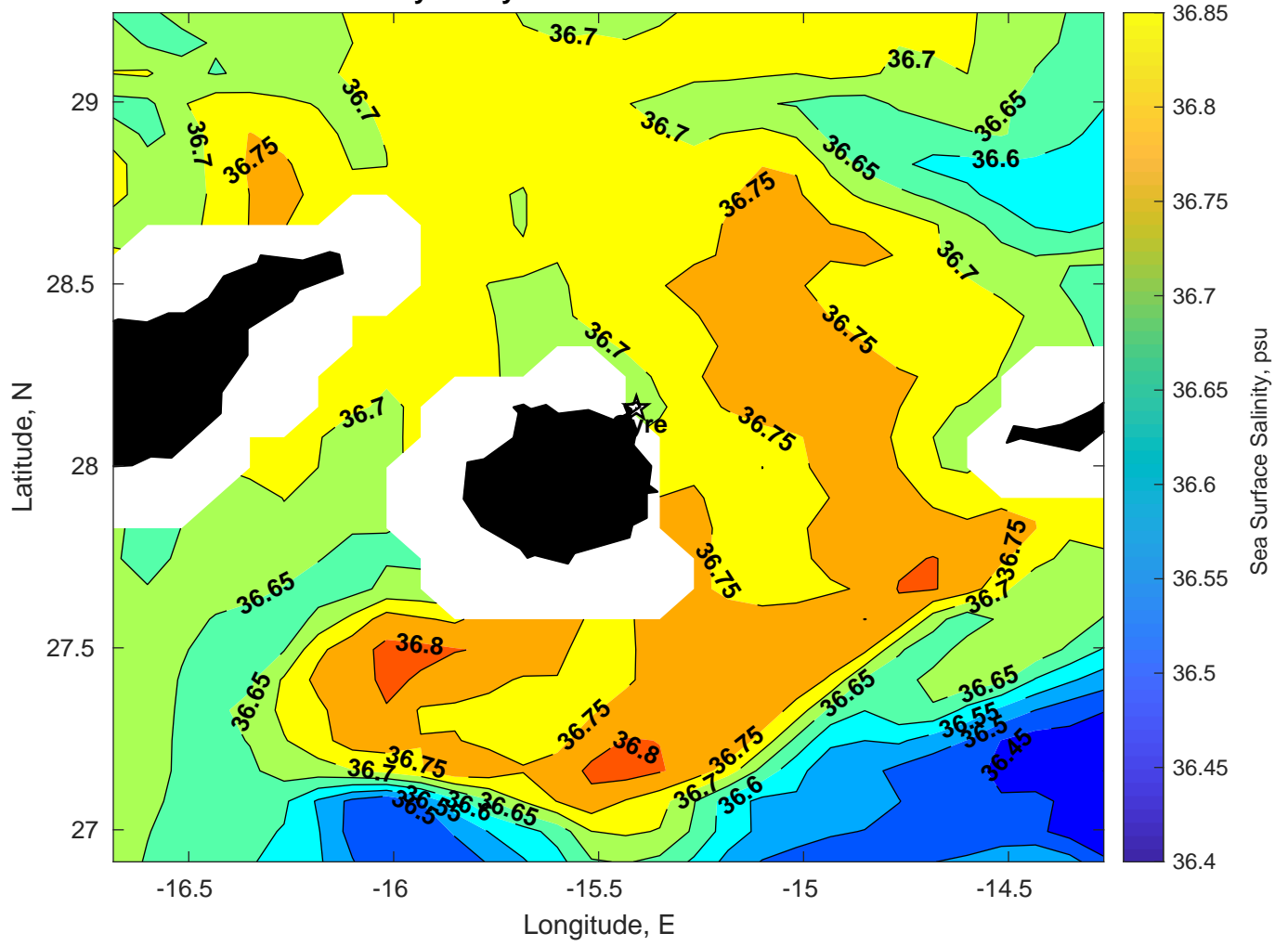
Surface Salinity for Gyre at 07-Feb-2025 00:00:00
