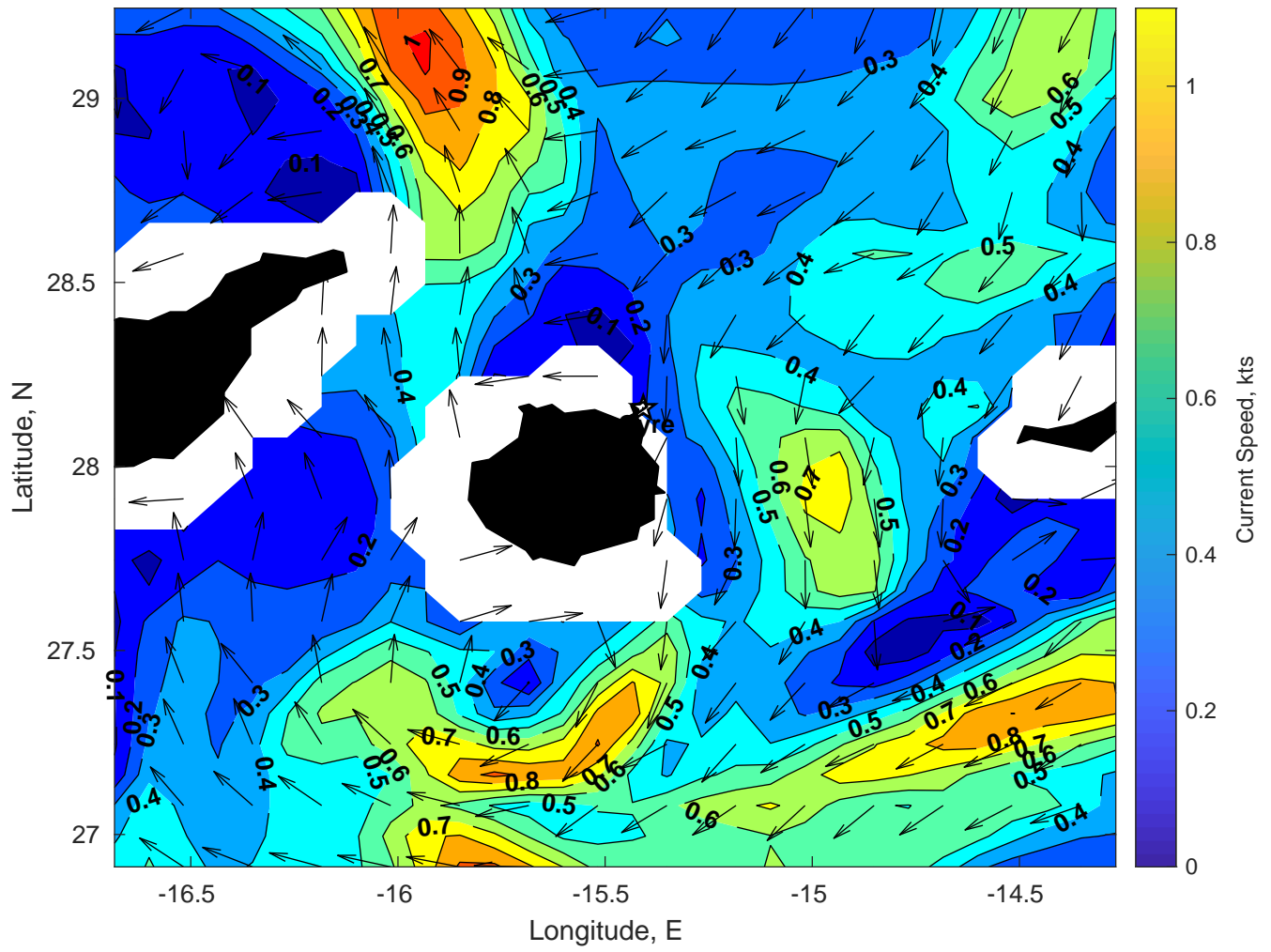
Surface Currents for Gyre at 07-Feb-2025 00:00:00
