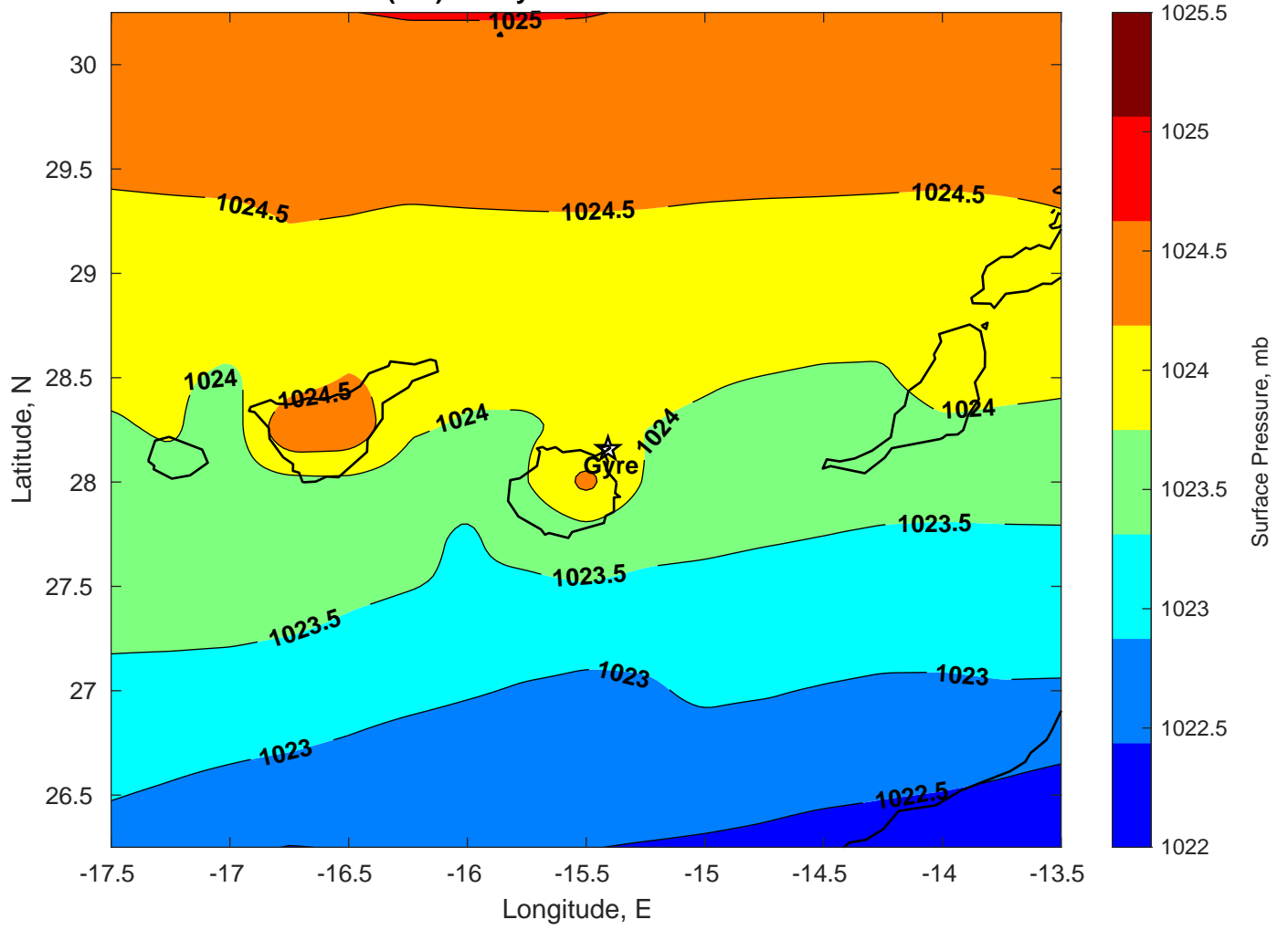
Surface Pressure (mb) for Gyre at 08-Feb-2025 00:00:00
