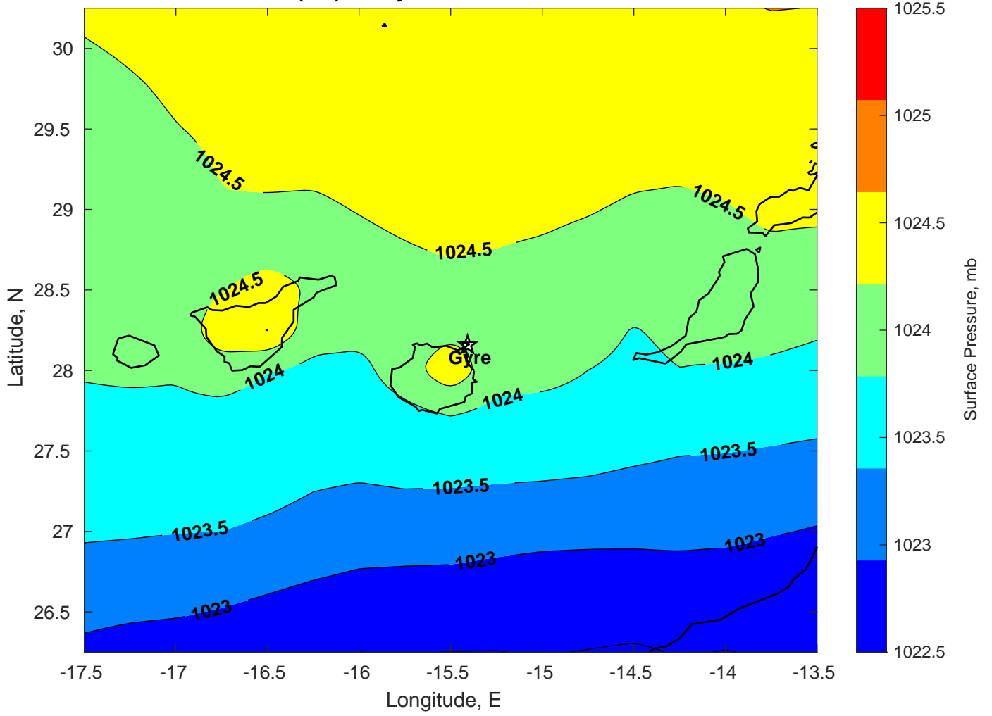
Surface Pressure (mb) for Gyre at 09-Feb-2025 00:00:00
