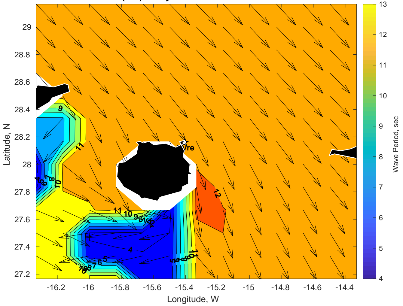
Wave Period (sec) for Gyre at 08-Feb-2025 09:00:00
