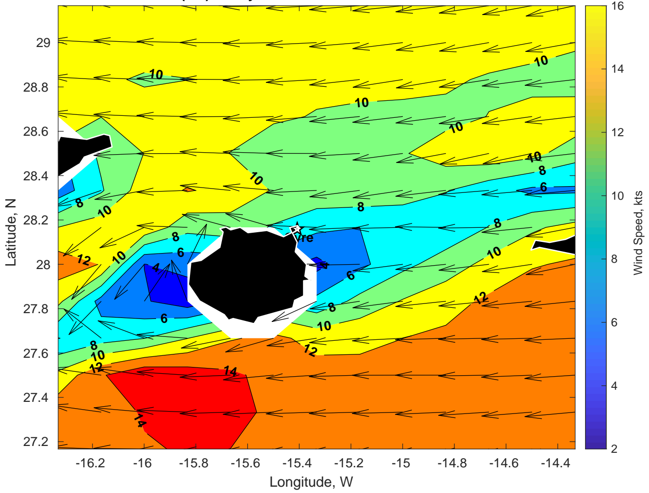
Winds (kts) for Gyre at 08-Feb-2025 09:00:00
