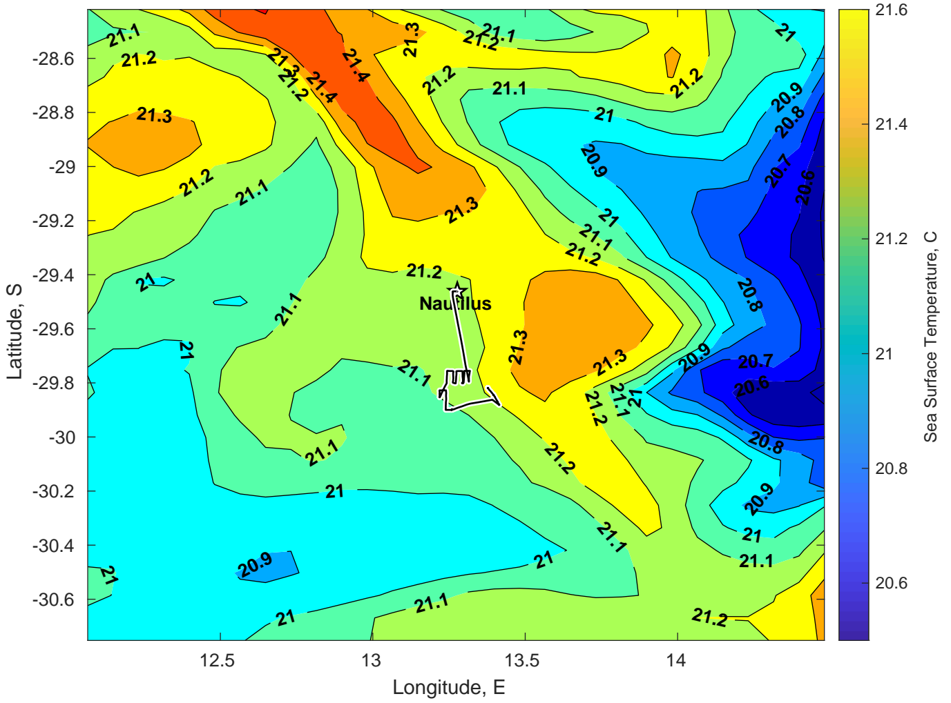
SST for Nautilus at 07-Feb-2025 00:00:00
