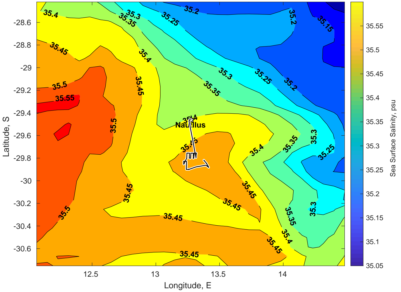
Surface Salinity for Nautilus at 07-Feb-2025 00:00:00
