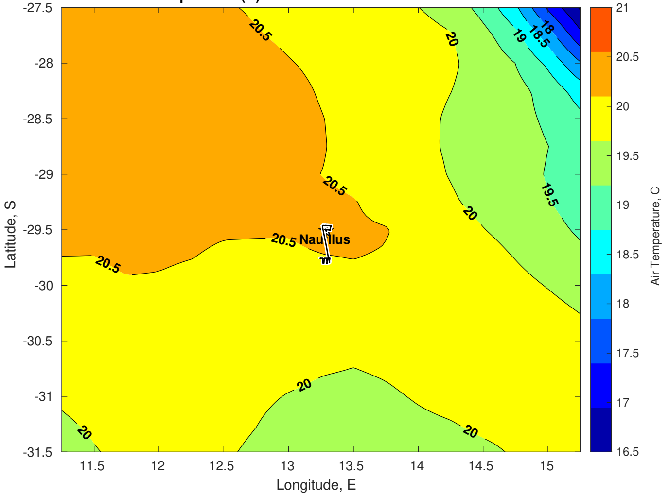
Air Temperature (C) for Nautilus at 08-Feb-2025
