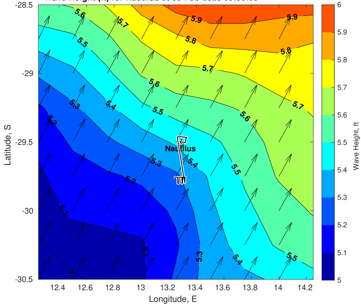
Wave Height (ft) for Nautilus at 08-Feb-2025 09:00:00
