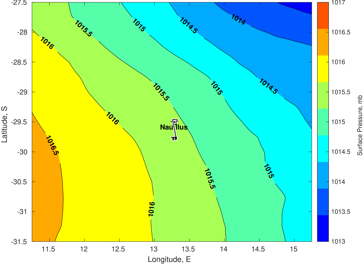
Surface Pressure (mb) for Nautilus at 08-Feb-2025 00:00:00
