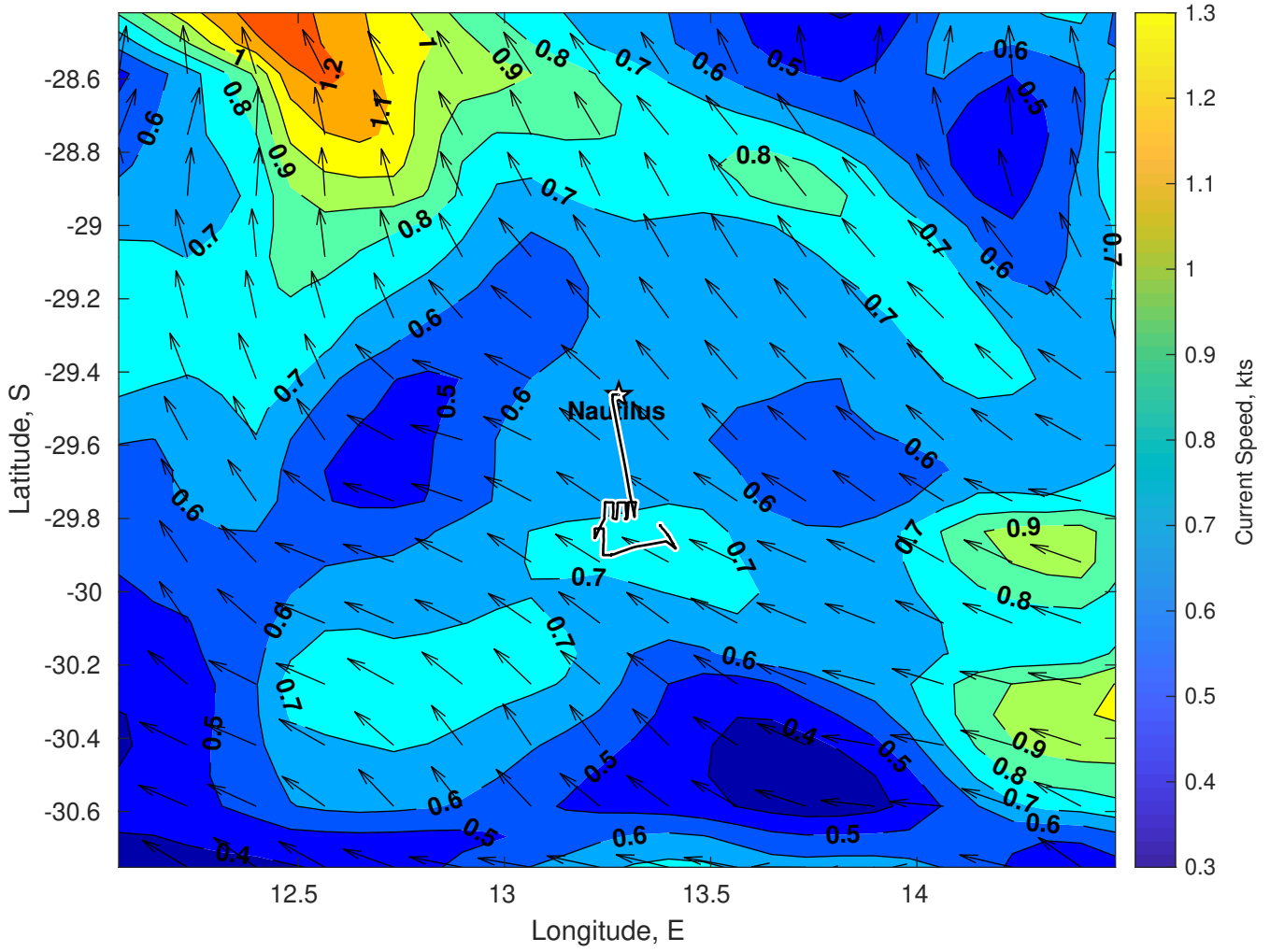
Surface Currents for Nautilus at 07-Feb-2025 00:00:00
