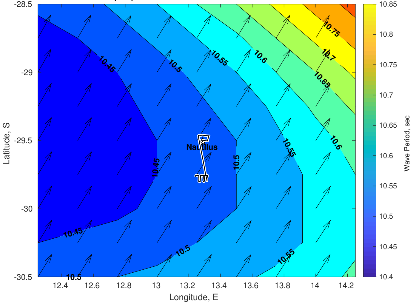
Wave Period (sec) for Nautilus at 08-Feb-2025 09:00:00
