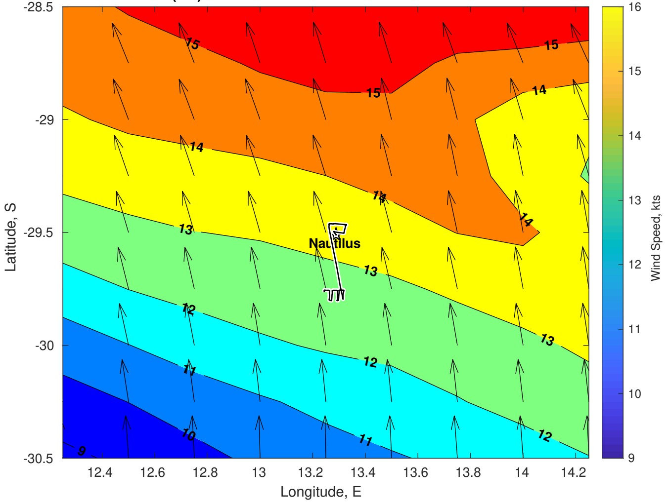
Winds (kts) for Nautilus at 08-Feb-2025 09:00:00
