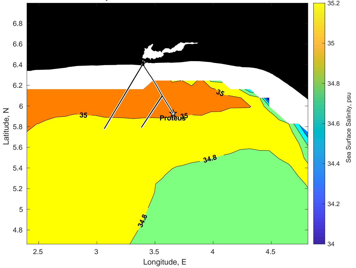
Surface Salinity for Proteus at 07-Feb-2025 00:00:00
