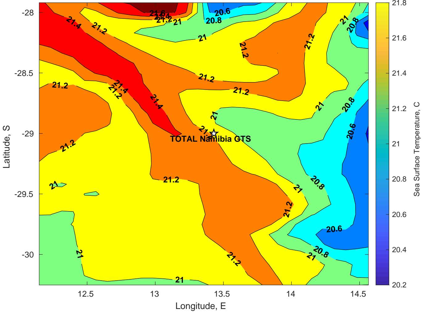
SST for TOTAL Namibia GTS at 07-Feb-2025 00:00:00
