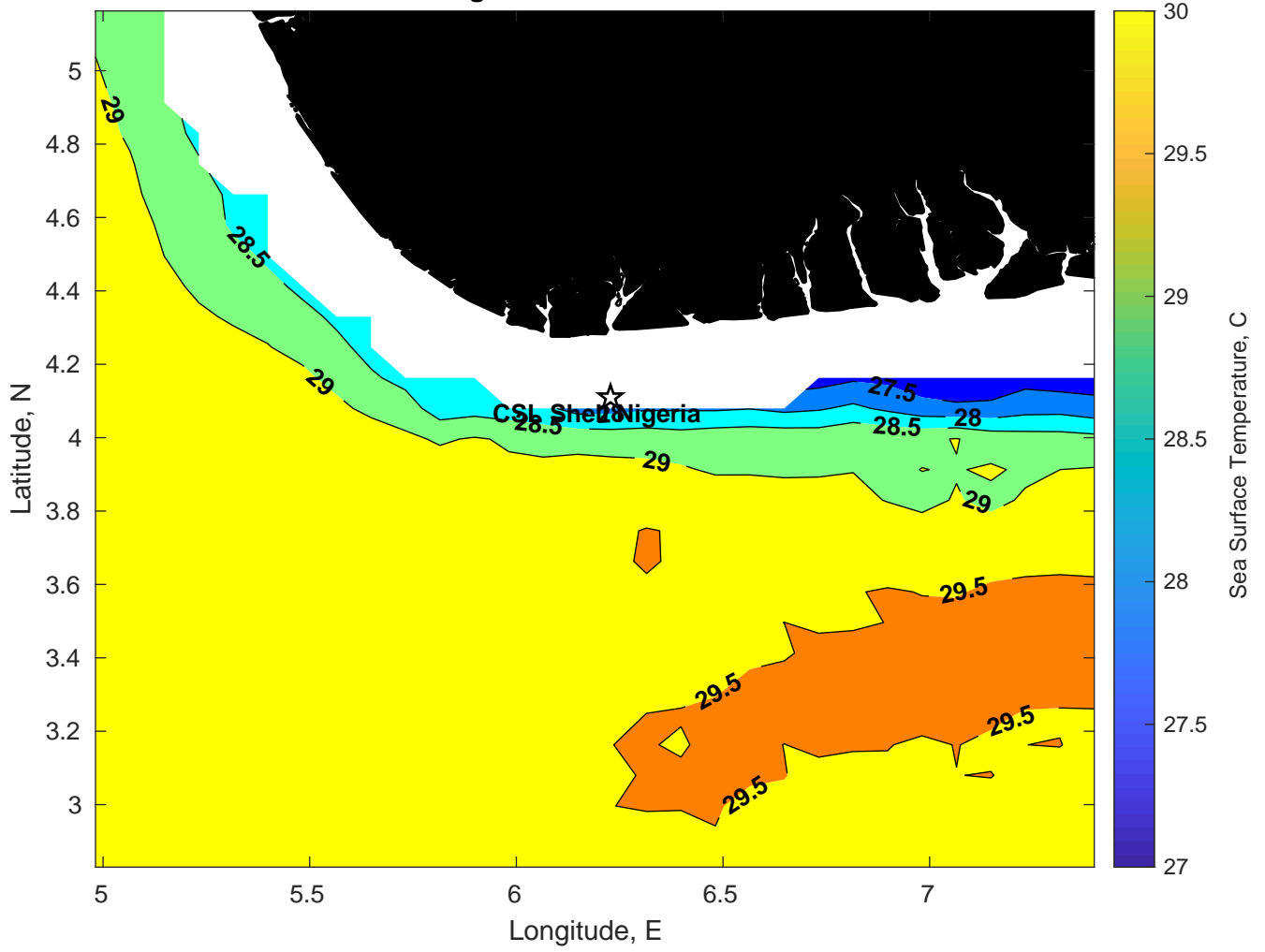
SST for CSL Shell Nigeria at 08-Feb-2025 00:00:00
