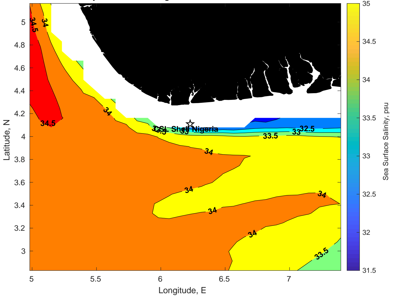
Surface Salinity for CSL Shell Nigeria at 08-Feb-2025 00:00:00
