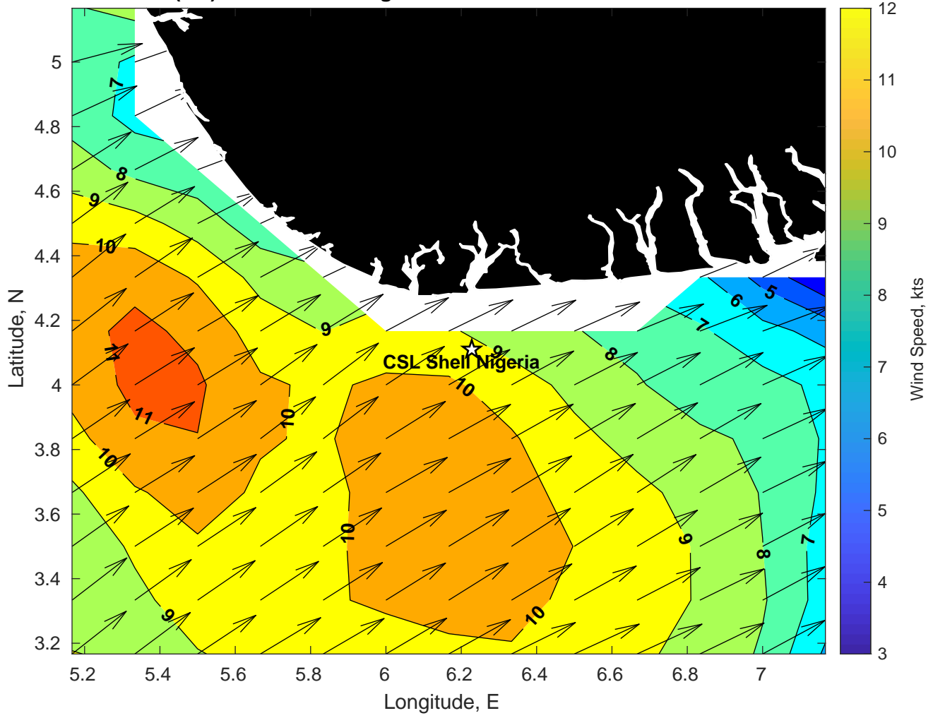
Winds (kts) for CSL Shell Nigeria at 09-Feb-2025 09:00:00
