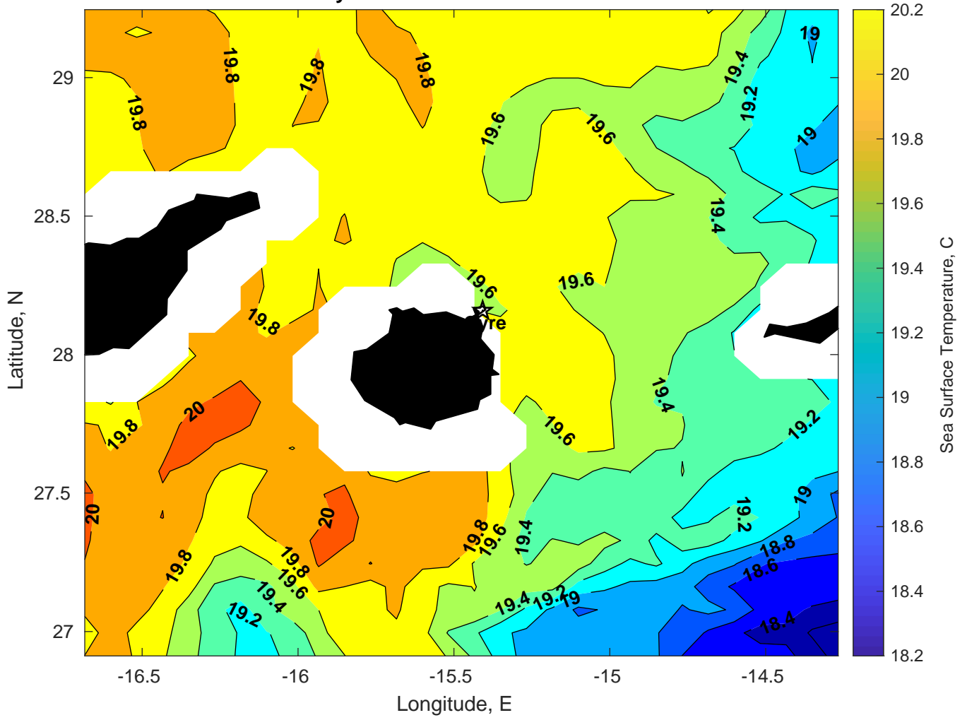
SST for Gyre at 08-Feb-2025 00:00:00
