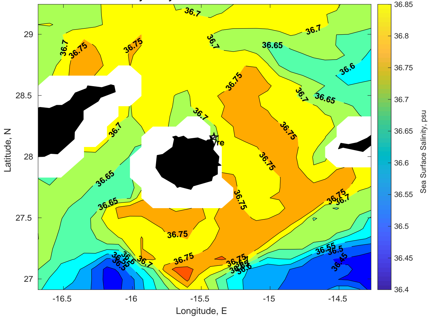
Surface Salinity for Gyre at 08-Feb-2025 00:00:00
