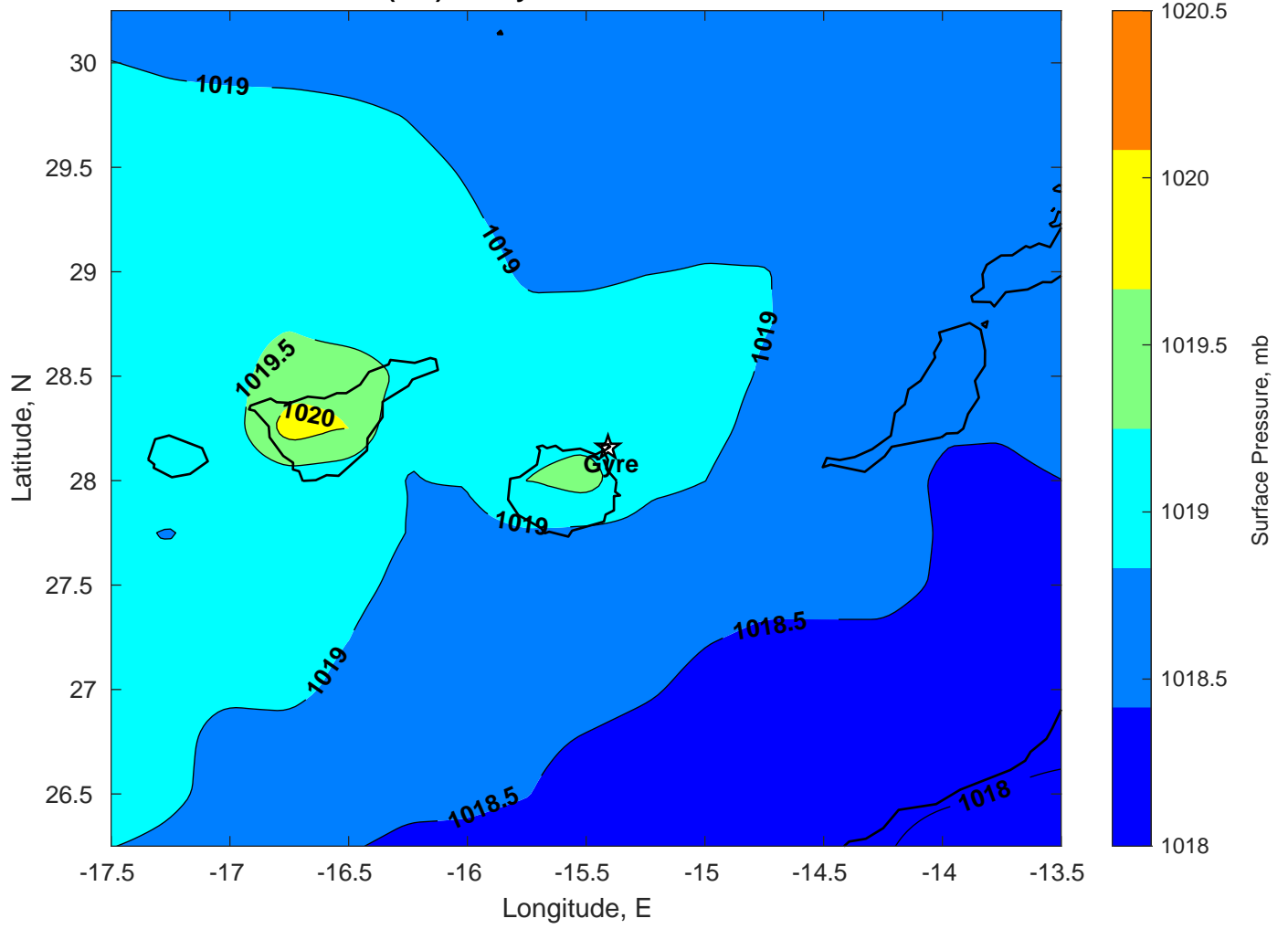
Surface Pressure (mb) for Gyre at 11-Feb-2025 00:00:00
